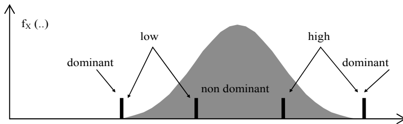
Figure 2: Dominant and non-dominant design values in a semi-probabilistic approach
