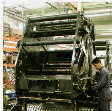
Assembly of the chain wheel.
