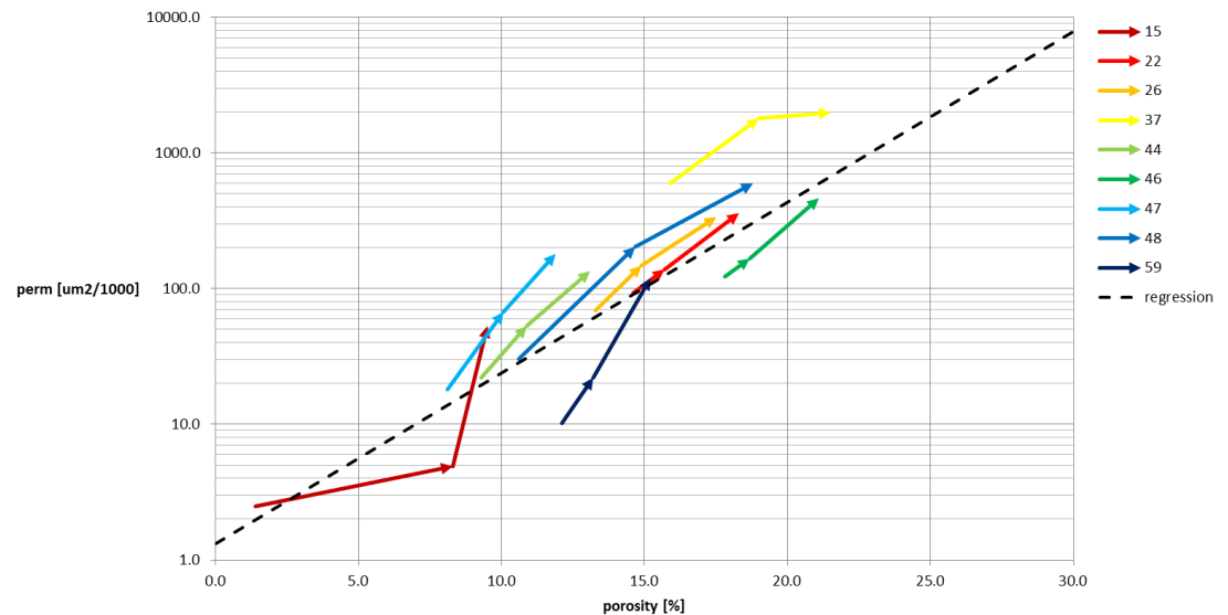
Figure 5.18 Porosity – permeability relationships of the acid stimulated KDZ-02 core plugs (also shown in Figure 5.17). Each colour arrow represents one core plug sample and two stimulation steps (first 15% HCl, second 12% HCl / 3% HF).
