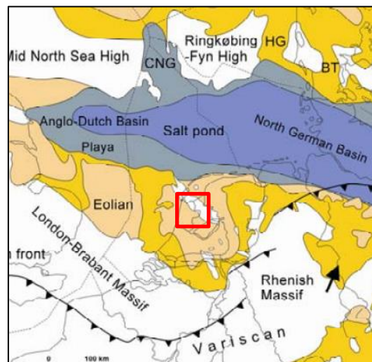
Figure 5.1 Facies and present-day distribution of Rotliegend sediments in the Permian Basin system. The study area (red box), located in a eolian dominated part of the area, lies at the southern flank of the Texel IJsselmeer High. Sketch (clipped to the Netherlands) from Geluk (2005).
