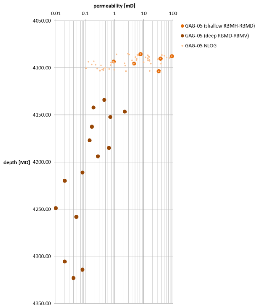
Figure 5.15 Permeability – depth relationship for the important GAG-05 well. RBMH = Hardegsen Formation, RBMD = Detfurth Formation, RBMV = Volpriehausen Formation. Note that in GAG-05 about 70 core plugs were measured (small dots). The large dots are the core plugs described in the NAM report 'GAAG-2A & GAAG-5 wells Sedimentology, petrography and reservoir quality of the Triassic Middle Buntsandstein' (source: NLOG)
