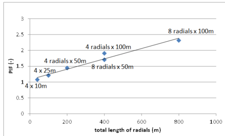
Figure 5.12 PIF for varying radials configurations as a function of the total length (number of radials × the length of a single radial)
