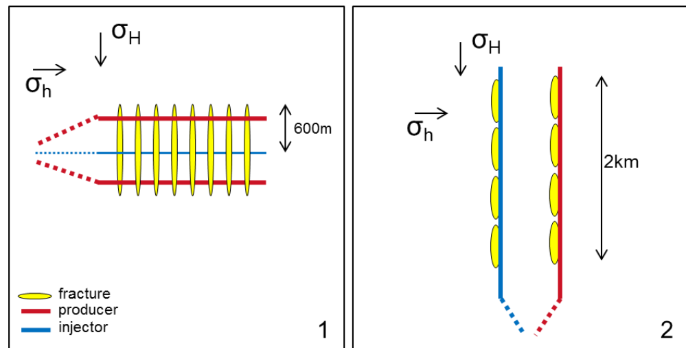
Figure 5.9 Schematic layout of sub-vertical fractures (top view) relative to wells. Scenario 1(left) marked by fractures perpendicular to the well bore is applicable when reservoir transmissivity is extremely low (hot dry rock; <0.5 Dm). Scenario 2 (right) marked by fractures oriented parallel to the fracture well is applicable when the transmissivity exceeds 0.5 Dm (after Pluymaekers et al., 2013).
