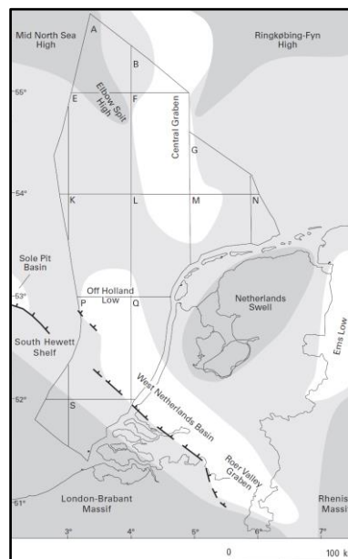
Figure 0.3 Triassic to Liassic structural elements (van Adrichem Boogaert and Kouwe 1997). Onshore, most sedimentation took place in the West Netherlands Basin and the Ems Low. Over the Netherlands Swell, sedimentation was absent or limited.
