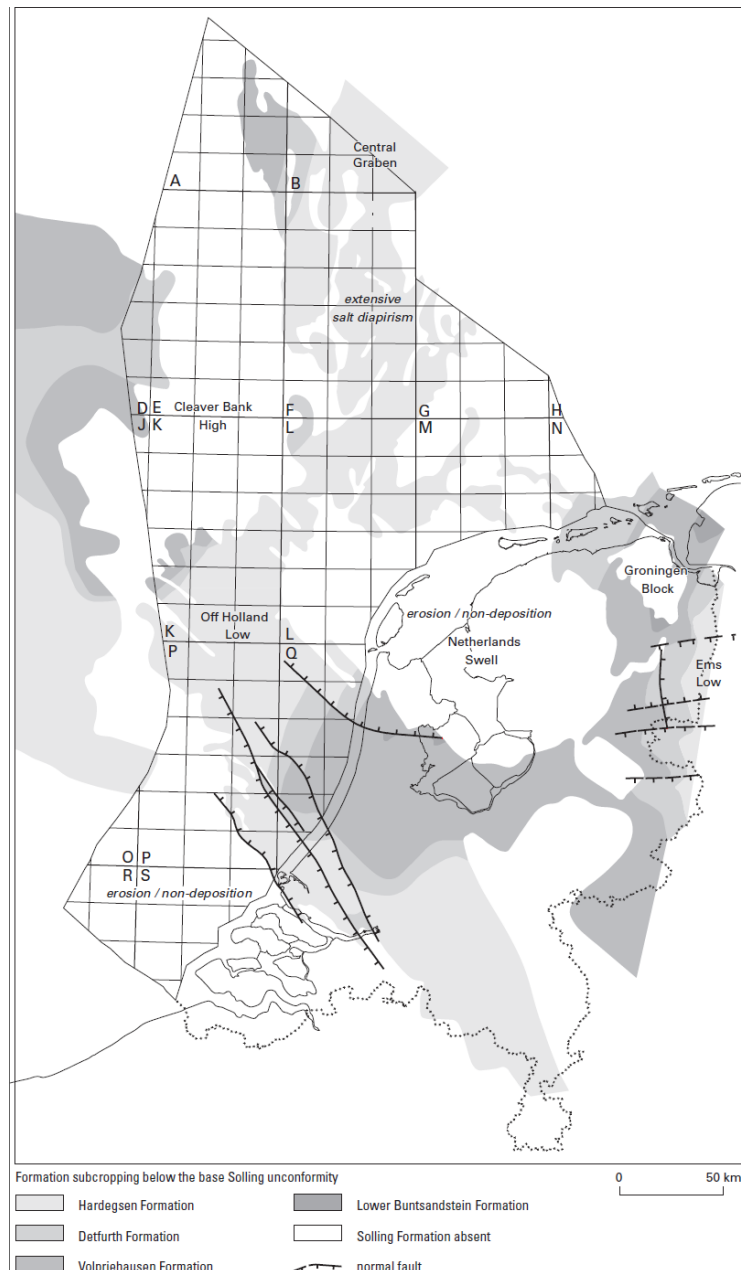
Figure 0.5 Formation subcrops below the Solling unconformity. In the more northern parts, the Volpriehausen Formation occurs, towards the south the Detfurth and Hardegsen (van Adrichem Boogaert and Kouwe 1997)
