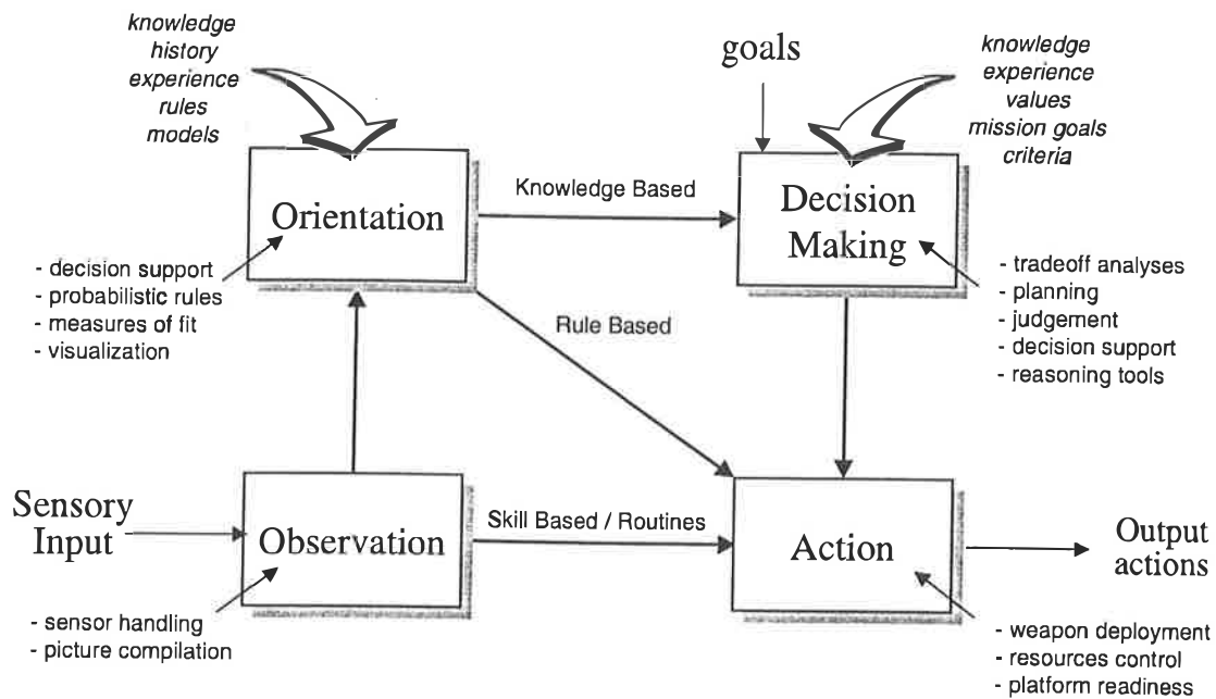
Figure 4. OODA cycle
