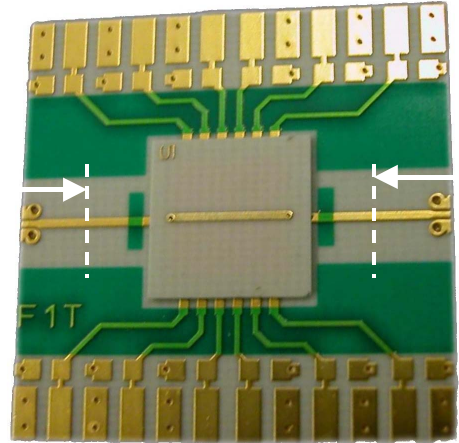
Fig. 5. Test structure for package through-line measurement.
