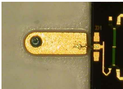
Fig. 7. Packaged HPA MMIC including barcaps.
