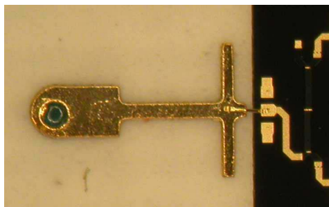
Fig. 8. Close-up of different bondwire compensation options: on the package and/or on-chip.
