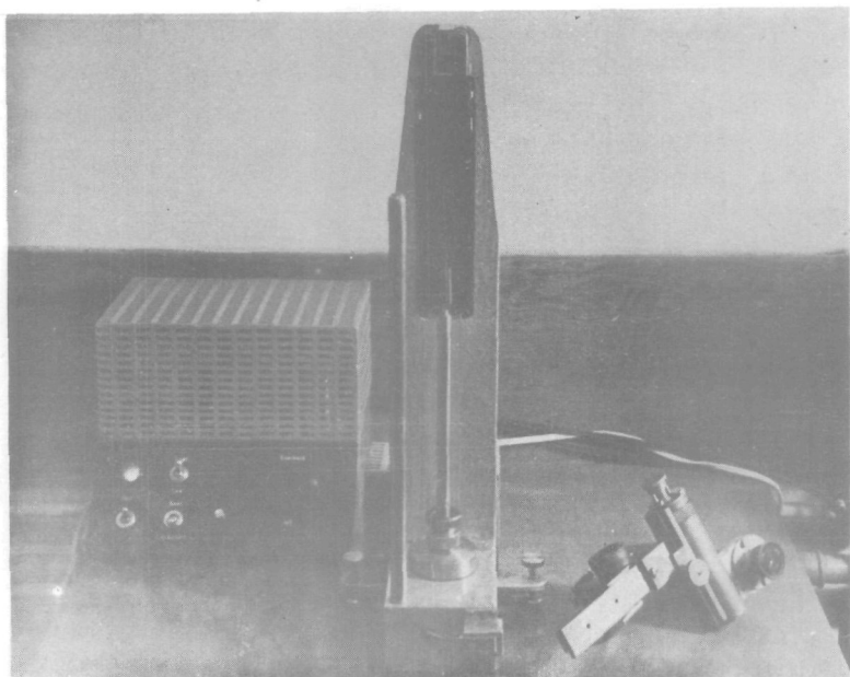
Fig. 20. General view of the apparatus for fibre friction
