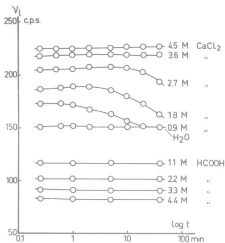
Fig. 39. Longitudinal resonance frequency as a function of time observed on one and the same wool fibre in several media
