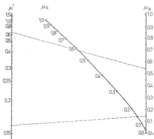
Fig. 29. Nomogram for the determination of \mu_k
