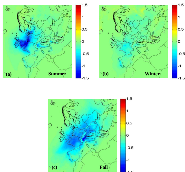
Figure 3. Predicted average change in ground-level concentrations ( \mu\text{g m}^{-3} ) of total PM 2.5 due to changes on gas/aerosol partitioning (based on a 2 K temperature increase) during the modeled (a) summer, (b) winter, and (c) fall periods. A positive value corresponds to an increase.
