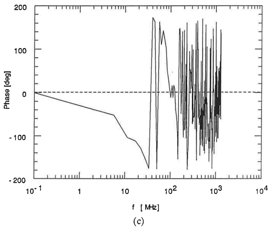
Figure 4.2 Incident H-field generated by the simulator. a) time domain, b) magnitude of the spectrum, c) phase of the spectrum.
