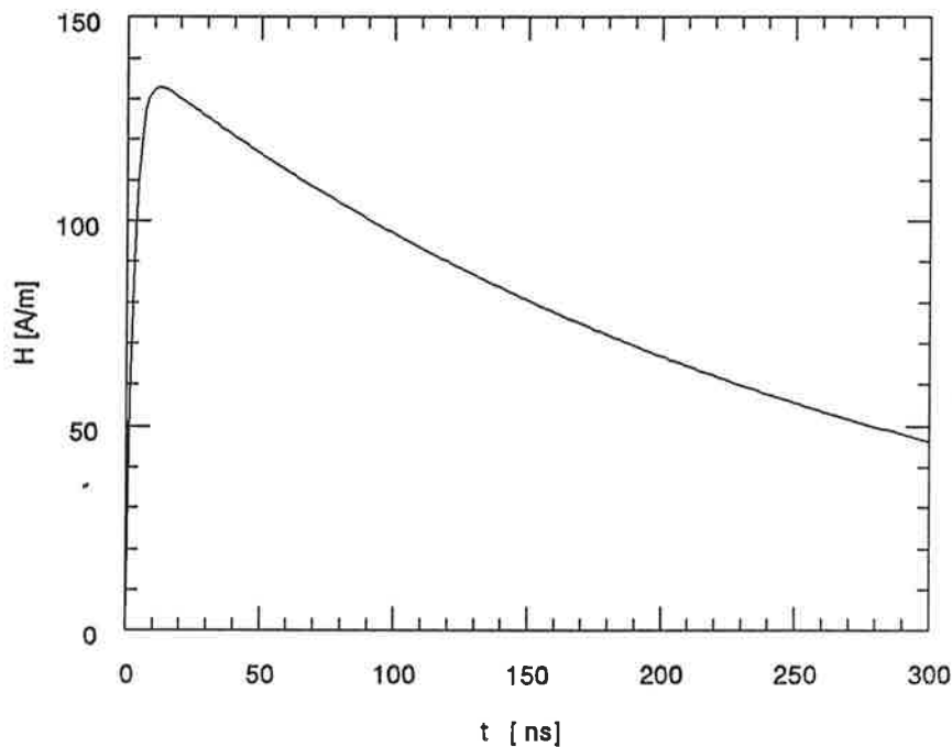
Figure 4.1 The prevailing waveform in the criterion environment.
