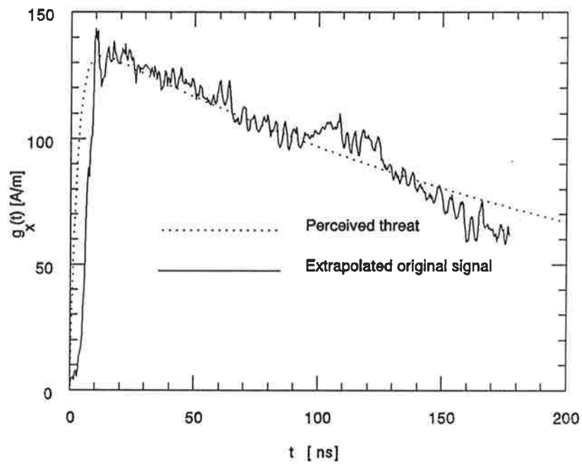
Figure 4.8 Result of the convolution of the extrapolation impulse response with the original signal of Figure 4.2.
