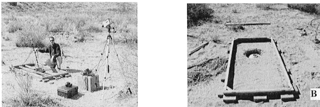
Figure 2: Field area with the ground penetration radar system at a frequency of 900 MHz and IR camera (A) and geometry of antitank landmine installation (B).
