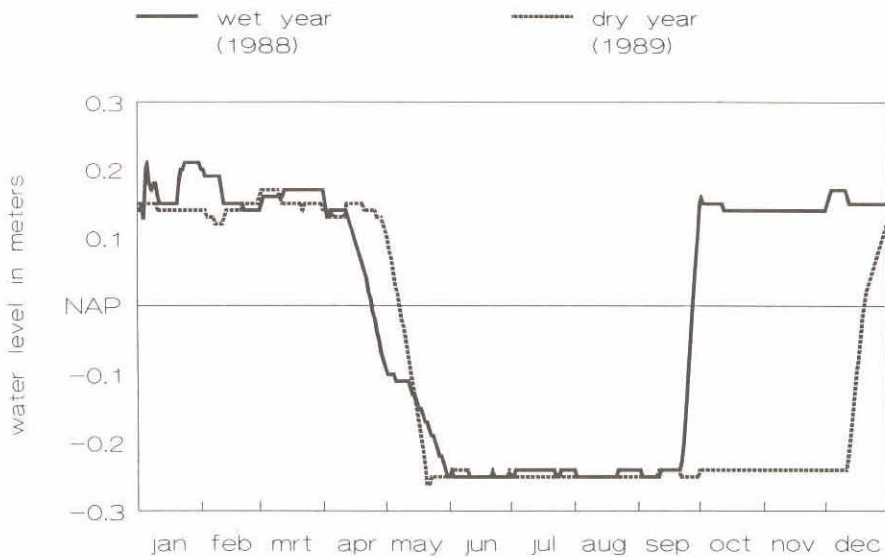
Figure 3 The water level if the control is effected at level margins of NAP + 15 cm and NAP - 25 cm
