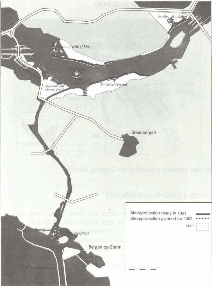
Figure 6 Shore defences already in place or planned before 1992
