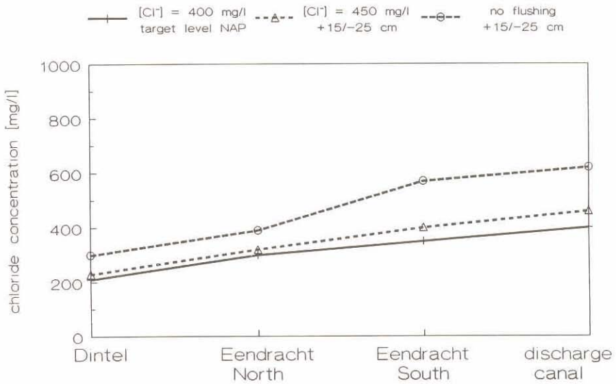
Figure 5 The chloride concentration at the different alternatives for the water management
