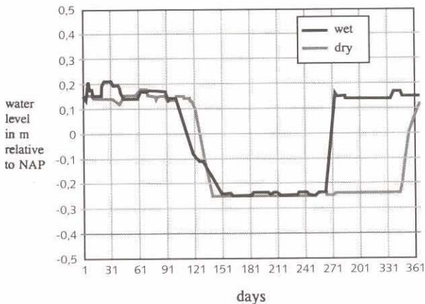
Figure 1 Fluctuations in water level in a wet (1988) and a dry (1989) year, with maximum and minimum at NAP + 0.15 m and NAP - 0.25 m
