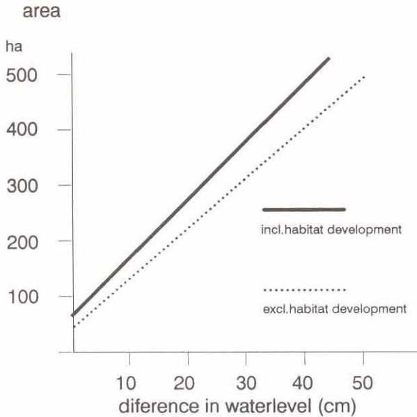
Figure 9 The more the shoreline can be extended, the greater the area affected by the water level
