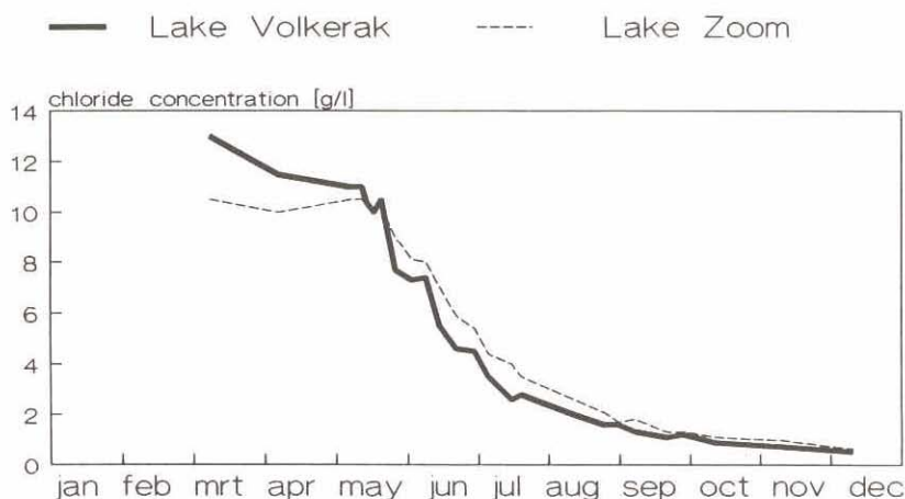
Figure 1 The desalination in 1987
