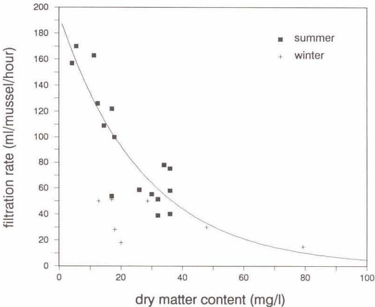
Figure 2 The effect of suspended matter content on filtration rate of Dreissena polymorpha . Lake IJsselmeer area, 1985 and 1988. Square symbols: values measured at water temperatures over 10°C; plus-signs: values measured at temperatures under 10°C.
