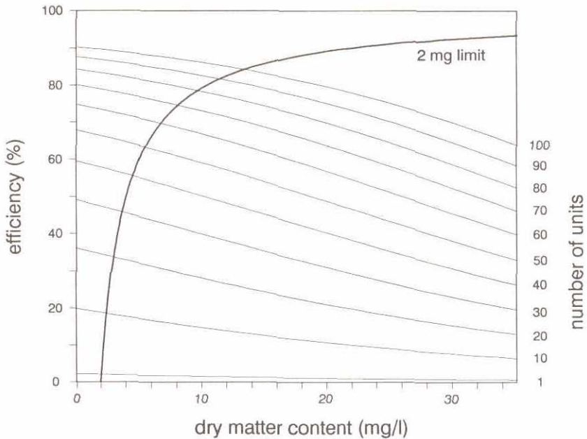
Figure 3 Efficiency of a biological filter out of different numbers of units (right axis), as a function of dry matter content. Water flow is 14 \text{ m}^3/\text{s} , mussel density on the nets is 5,000/\text{m}^2 . In practice, when dry matter content falls below 2 \text{ mg/l} , filtration decreases (see text).
