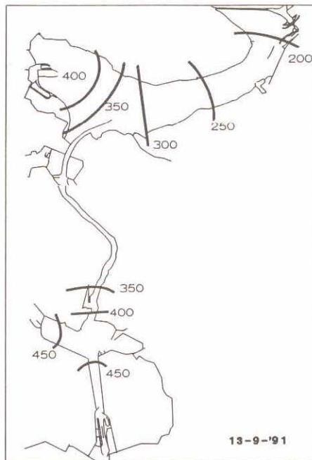
Figure 2 The chloride concentrations in Lake Volkerak/Zoom (mg/l)
