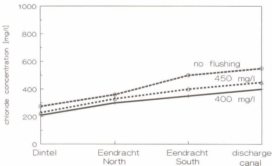
Figure 4 The chloride concentration at the different alternatives for flushing
