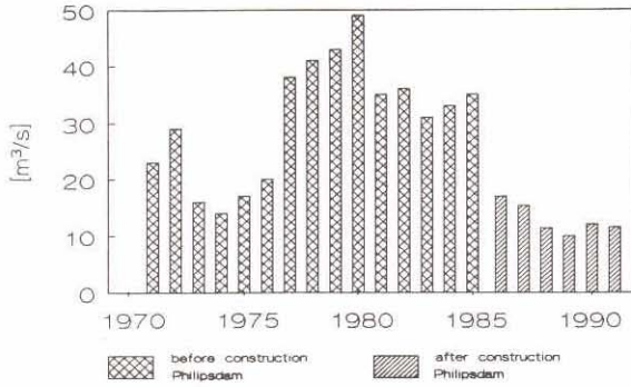
Figure 2 Flow through Volkerak sluices 1971-1991
