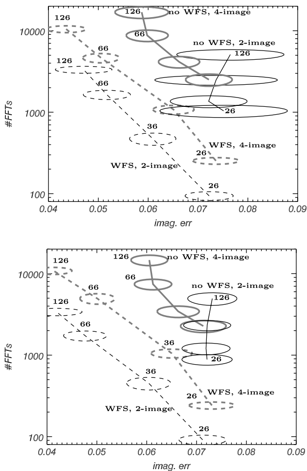
Fig. 3. The number of required FFTs as a function of reconstruction error. Solid lines show the pure PD; dashed lines are made with additional WF information. Thin lines are made with 2-image PD, thick lines with 4-image PD. The lines connect points with 26–126 estimated modal coefficients with the other simulation parameters fixed. The circles around the points show the rms computed over 32 random WF realizations and nine different subimages of the object. Upper plot: Kolmogorov-style turbulence ( r_0 = 0.08 m at 0.5 \mu\text{m} ). Seeing-limited image error \epsilon_s \approx 0.11 . Lower plot: WFs typical for an AO system. AO-corrected image error \epsilon_s \approx 0.09 .
