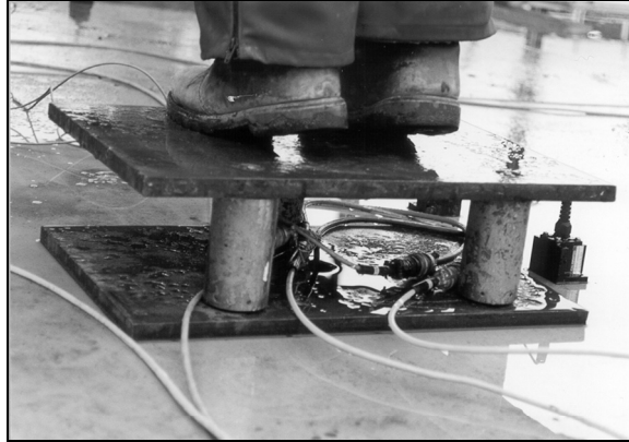
Figure 2: Load source heel drop, measured with load cells
