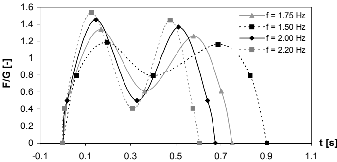
Figure 4: Vertical loads for several pace frequencies
