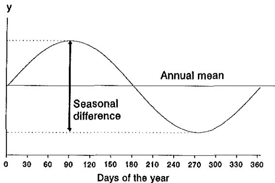
Figure 2.1.1 Seasonal curve for a hypothetical outcome variable.
