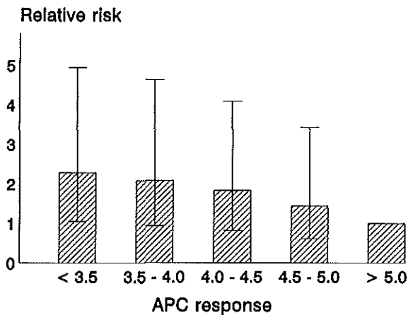
Figure 4.4.1 Relative risk of stroke and TIA according to level of APC response (adjusted for age and gender).
