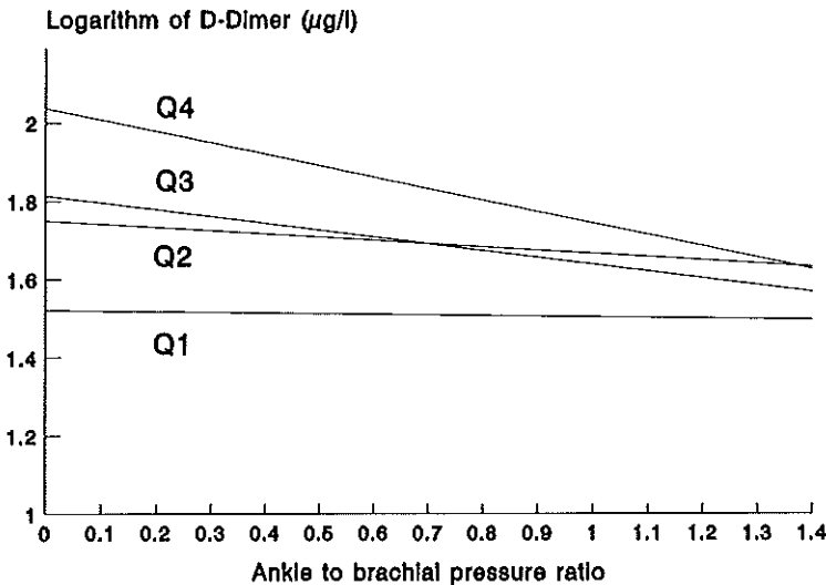
Figure 3.1.2. Regression lines for subgroups consisting of subjects in the 4 quartiles (Q1, Q2, Q3, and Q4) of the distribution of F1+2 (Cutpoints 1.54, 1.90, 2.39 \mu\text{g/l} ), adjusted for age and sex.
