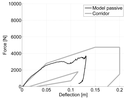
Figure12. PMHS response corridors and active human model (passive) response in blunt frontal abdomen impact 31.4 kg at 6.9 m/s.
