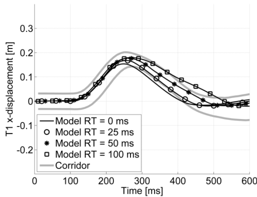
Figure16. T1 x-displacement w.r.t. sled of active human model at various RT's and CCR=0.5 and volunteer response corridors in 3.8 g frontal impact.
