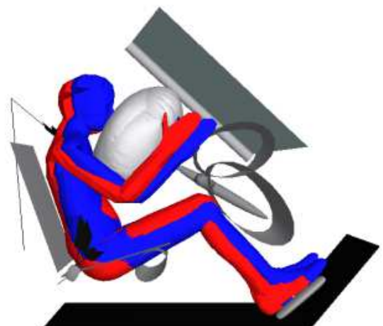
Figure24. Position of the active model with (blue) and without (red) preceding braking at 1060 ms of the frontal impact simulations of the small car.
