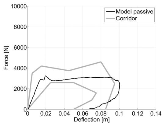
Figure8. PMHS response corridors and active human model (passive) response in blunt frontal thorax impact with 23.4 kg at 6.9 m/s.
