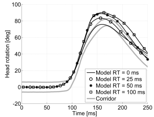
Figure18. Head rotation w.r.t. to sled of active human model at various RT's and CCR=0.5 ms and volunteer response corridors in 15 g frontal impact.
