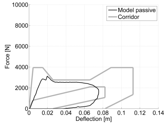
Figure10. PMHS response corridors and active human model (passive) response in blunt frontal thorax impact with 10.4 kg at 7 m/s.
