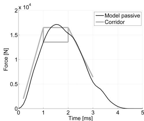
Figure4. PMHS response corridors and active human model (passive) response in blunt frontal head impact with 23.4 kg at 5.5 m/s.
