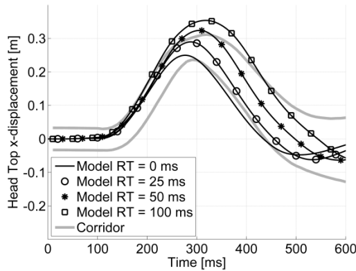
Figure15. Head top x-displacement w.r.t. sled of active human model at various RT's and CCR=0.5 and volunteer response corridors in 3.8 g frontal impact.
