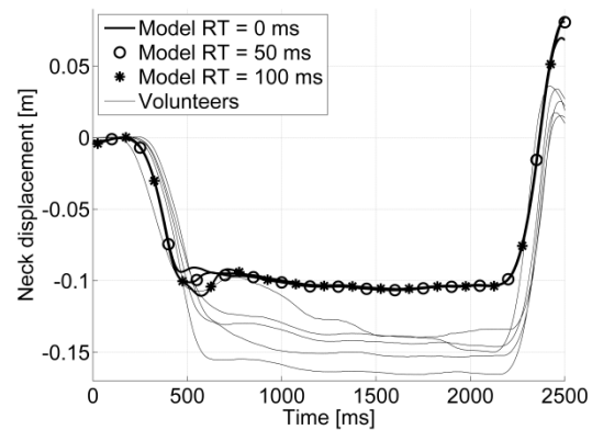
Figure14. Neck displacement of active human model at various RT's and CCR=0.5 and of volunteers in 1 g car braking.
