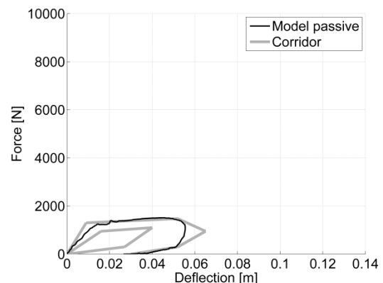
Figure5. PMHS response corridors and active human model (passive) response in blunt frontal thorax impact with 23.4 kg at 3.4 m/s.
