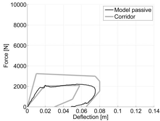
Figure7. PMHS response corridors and active human model (passive) response in blunt frontal thorax impact with 23.4 kg at 4.9 m/s.
