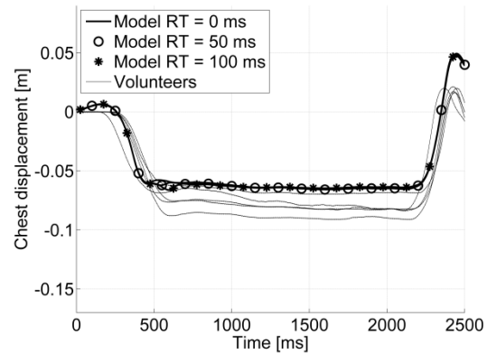
Figure13. Chest displacement of active human model at various RT's and CCR=0.5 and of volunteers in 1 g car braking.
