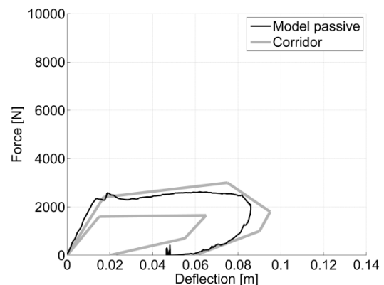
Figure6. PMHS response corridors and active human model (passive) response in blunt frontal thorax impact with 23.4 kg at 5.8 m/s.
