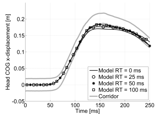
Figure19. Head COG x-displacement w.r.t. sled of active human model at various RT's and CCR=0.5 and volunteer response corridors in 15 g frontal impact.
