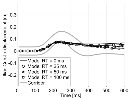
Figure17. Iliac crest x-displacement w.r.t. sled of active human model at various RT's and CCR=0.5 and volunteer response corridors in 3.8 g frontal impact.
