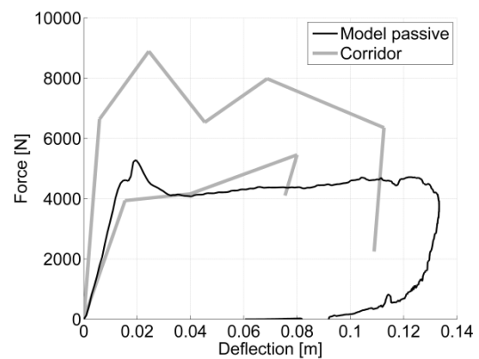
Figure11. PMHS response corridors and active human model (passive) response in blunt frontal thorax impact with 22.2 kg at 9.9 m/s.
