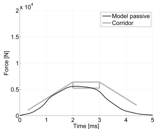
Figure3. PMHS response corridors and active human model (passive) response in blunt frontal head impact with 23.4 kg at 2 m/s.
