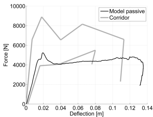
Figure9. PMHS response corridors and active human model (passive) response in blunt frontal thorax impact with 23.4 kg at 9.9 m/s.
