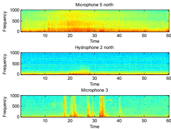
Figure 4: Spectrograms of microphone and hydrophone signals during collapse of the dike.
