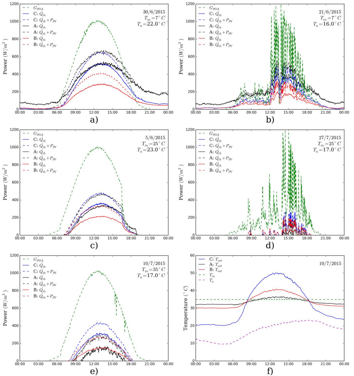
Fig 2. Graphs 2a to 2e show the in-plane irradiance (green dashed lines), the heat flow (continuous lines) and the heat flow plus PV power (added with dashed lines) for five different days with different return/input temperatures (a&b) 7^\circ C , (c&d) 25^\circ C and (e&f) 35^\circ C . Figure 2f shows the ambient temperature (purple), the input/return temperature and the flow/output temperature for each system. The colours refer to: Blue: system C, Black: system A, Red: system B. The average ambient temperature is written in each subfigure.
