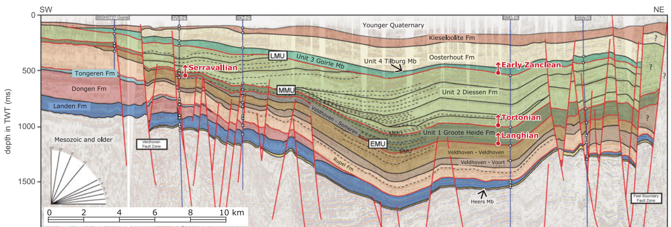
Figure 7. Geological interpretation of the lithostratigraphical units in the RVG by integrated multidisciplinary results.
