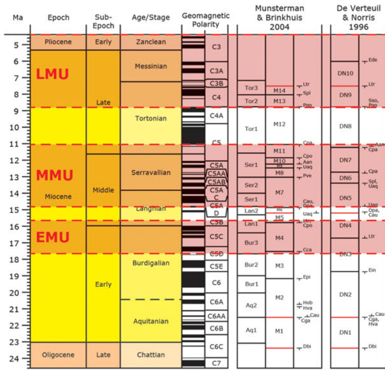
Figure 11. (Early Miocene–Mid-Miocene–Late Miocene) Unconformities deduced from well G11-1, German North Sea Sector (adjusted after Köthe et al., 2008).
