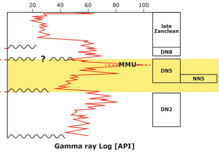
Figure 11. (Early Miocene–Mid-Miocene–Late Miocene) Unconformities deduced from well G11-1, German North Sea Sector (adjusted after Köthe et al., 2008).
