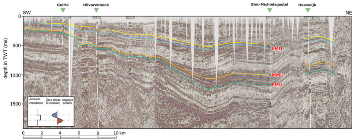
Figure 6. Seismic interpretation of a NE-SW (c. perpendicular) transect in the RVG, including wells Heeswijk-01 (HSW-01), St-Michielsgestel-01 (SMG-01), Hilvarenbeek-01 (HVB-01) and Goirle (50H0373).
