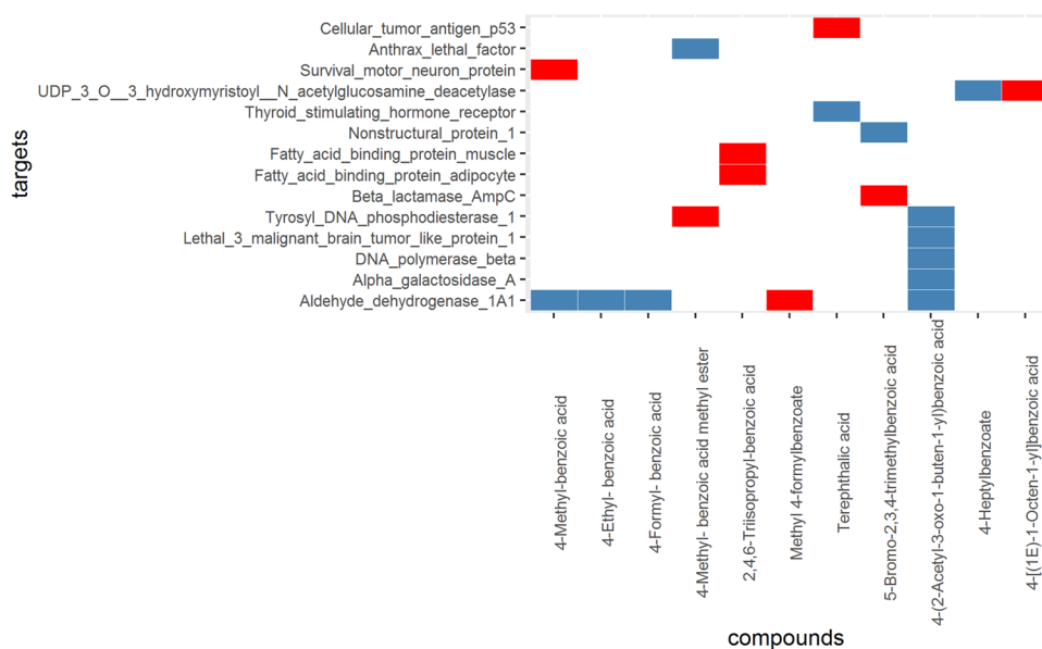
Fig. 6 A heat map showing the pharmacological pattern of 4-methylbenzoic acid and ten structurally most similar analogues extracted from ChEMBL (version 24). Red cells indicate active measurements; blue cells indicate inactive measurements (cutoff set to 10 \mu M) (color figure online)
