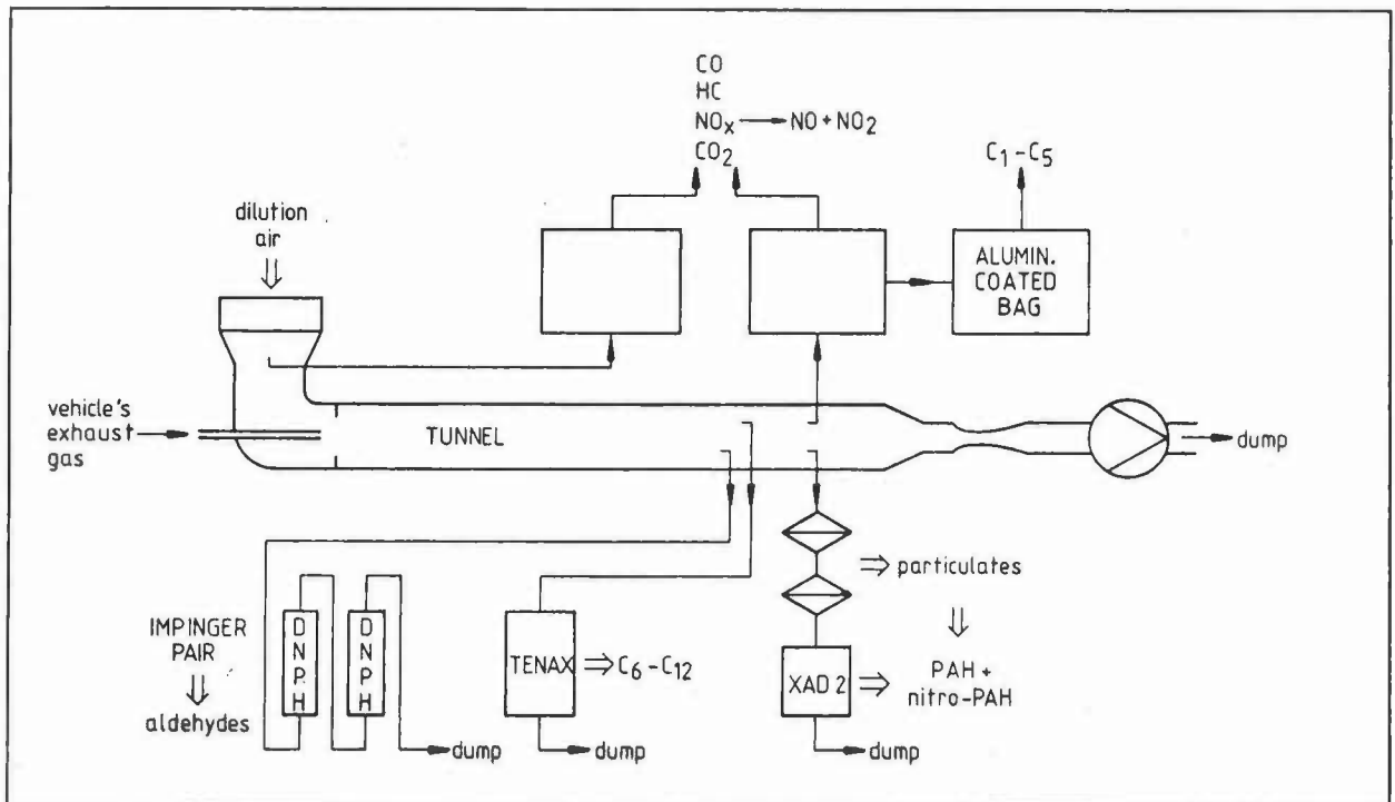
Figure 3.2: Adapted CVS sampling system (regulated and unregulated components)
