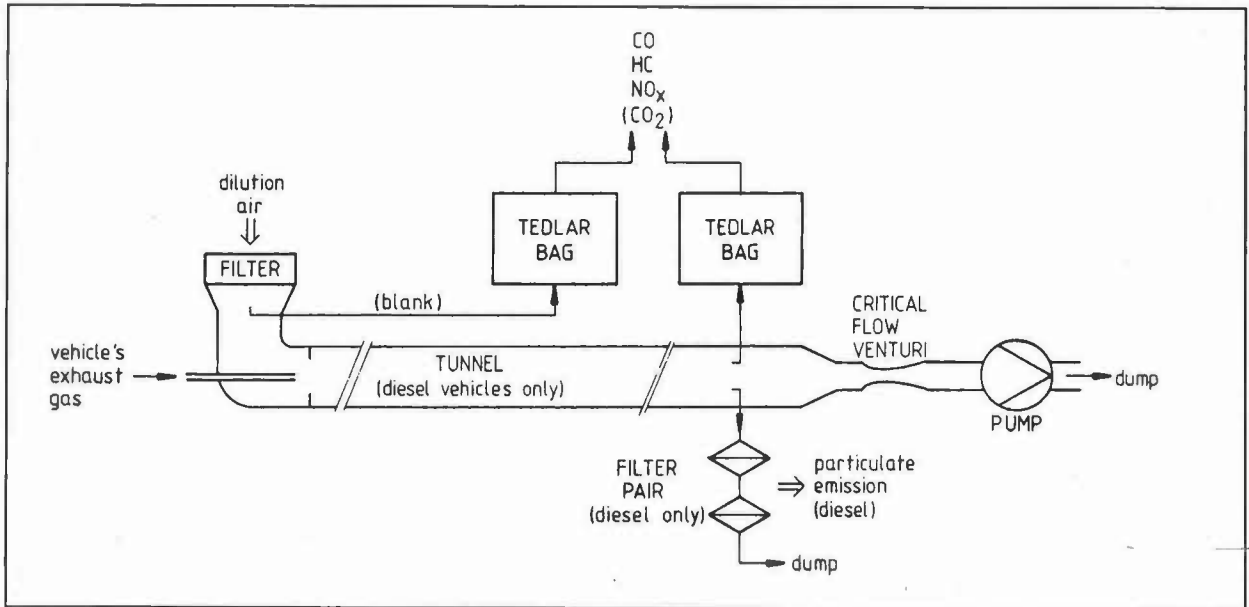
Figure 3.1: Conventional CVS sampling system (regulated components)
