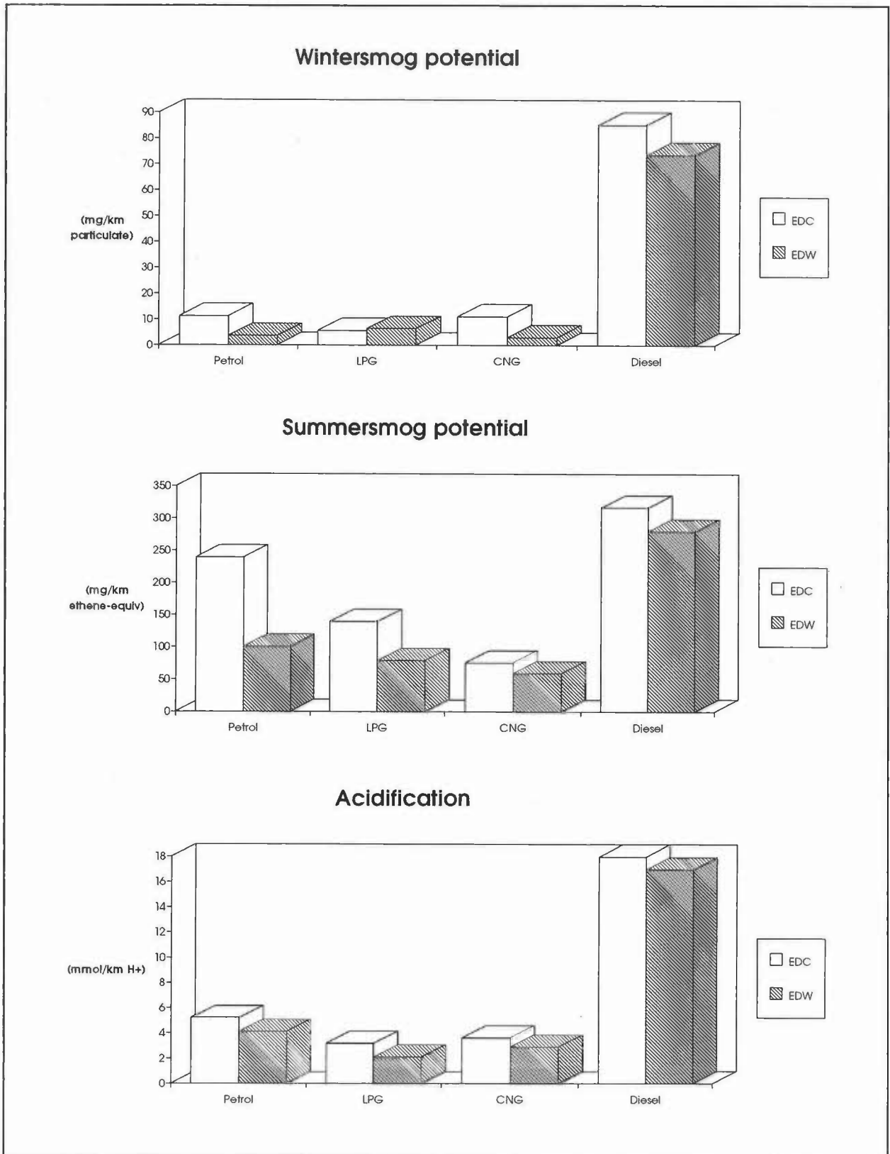
Figure 6.3a: Coldstart effects on regional and global effects
