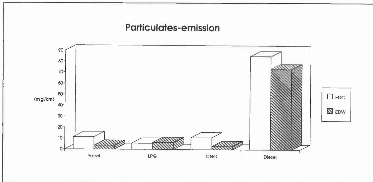
Figure 6.1b: Coldstart effects on direct toxic components (concluded)
