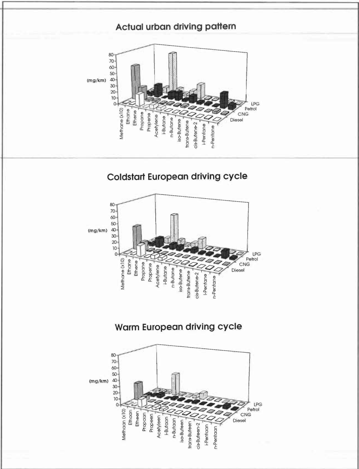
Figure 4.4a: Emission of light hydrocarbons (C 1 -C 5 )
