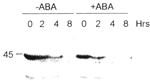
Fig. 2. Effect of ABA on MBP phosphorylating activity in embryos during imbibition of barley grains. Intact grains were treated with 100 \mu M ABA. embryos were isolated at designated times and in-gel kinase analysis was performed as described for Fig. 1A. 30 \mu g of protein was loaded. One representative example of four independent experiments is presented.
