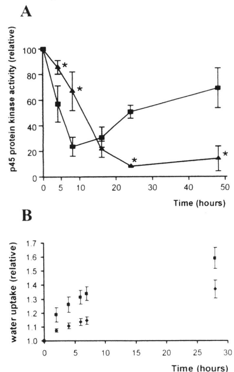
Fig. 3. MBP kinase activity and water uptake in non-dormant and dormant barley grains. (A) In-gel MBP kinase analysis as described in Fig. 1A. ■, non-dormant grains; ▲, dormant grains. Activity of the 45 kDa MBP phosphorylating activity (p45 protein kinase) was quantified using ImageQuant (Molecular Dynamics). Data are the mean of three independent experiments. (*) indicates significant difference with non-dormant grains, as determined with the Student's t -test ( P < 0.05 ). (B) Water uptake of intact non-dormant (■) and dormant (◆) barley grains. Water uptake was determined by weighing individual grains repeatedly during imbibition. Two independent experiments with in total 20 non-dormant and 20 dormant grains are presented. The mean values \pm S.D. of 20 individual grains are shown.
