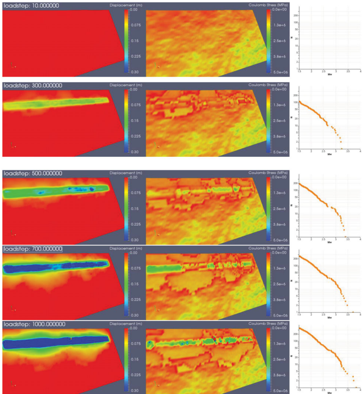
Fig. 13. Rupture model results of 25 MPa pressure depletion for finite element stresses for 0.5D model with ambient pressure, with close to critical in situ stress ( K_{0\text{eff}} = 0.4 ).
