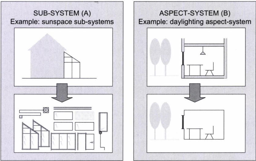
Figure 2.1: Sub-system view (A) versus aspect-system view (B)
