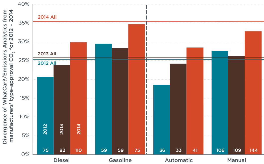
Figure 20. Divergence of WhatCar? /Emissions Analytics data from official CO 2 emission values for 2012 to 2014 by fuel and transmission type. The number of entries are presented at the base of each column. The average divergence of all vehicles (including hybrids) for each year is also presented.
