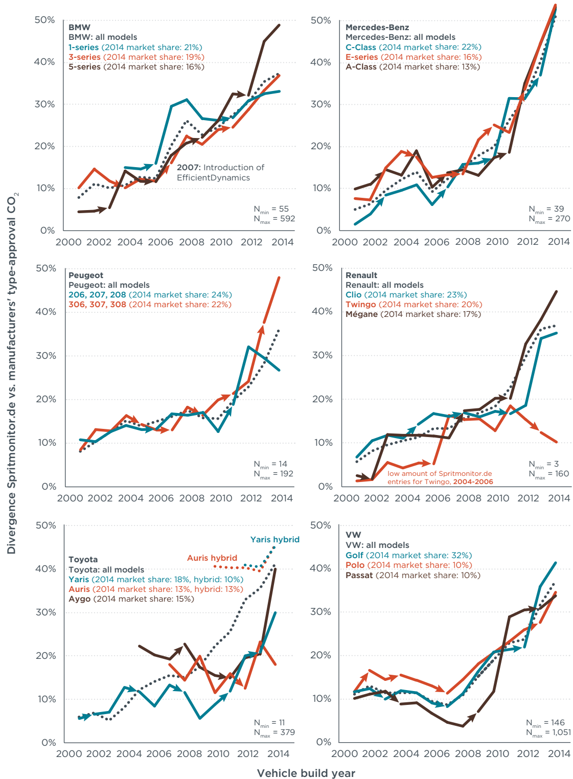
Figure 9. Divergence of Spritmonitor.de data from manufacturers' type-approval CO 2 emissions by brand and by top-selling models 14 .
