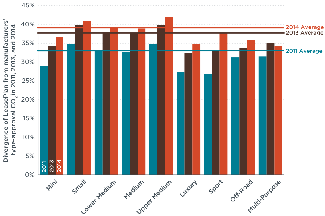
Figure 14. Divergence of LeasePlan data from manufacturers' type-approval CO 2 emissions by segments for 2011, 2013, and 2014.
