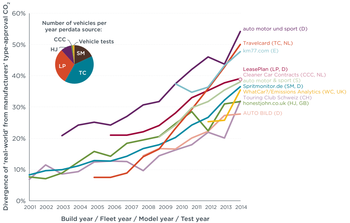
Figure 25. Divergence of real-world from manufacturers' type-approval CO 2 emissions for various on-road data sources.
