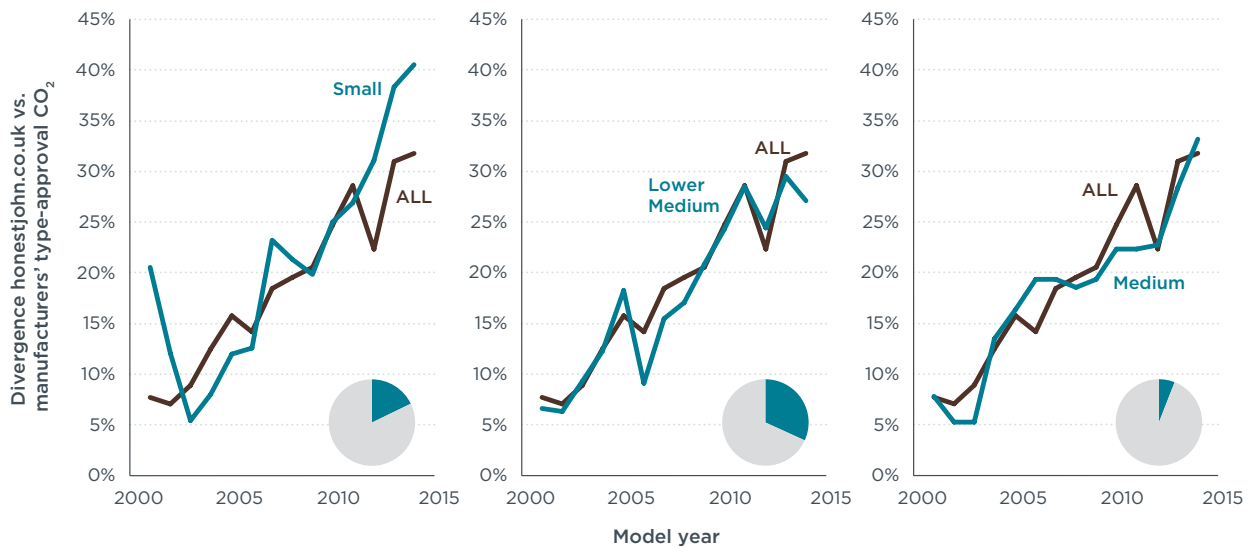
Figure 17. Divergence of honestjohn.co.uk data from manufacturers' type-approval CO 2 emissions by vehicle segment (pie chart indicates share of segments in the data set for 2014).
