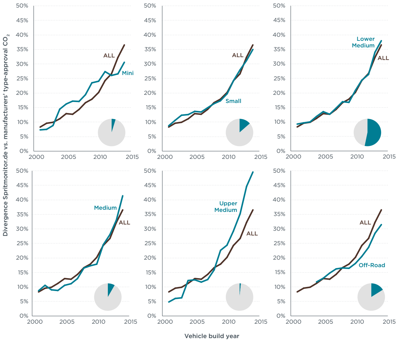
Figure 7. Divergence of Spritmonitor.de from manufacturers' type-approval values by vehicle segment (pie chart represents the share of vehicles per segment in the data set for 2014).
