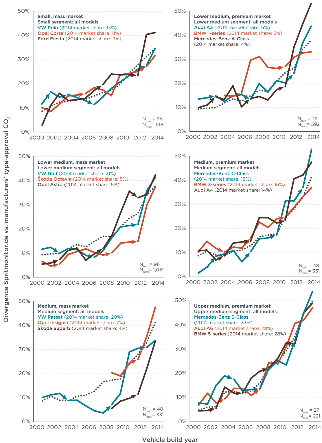
Figure 10. Divergence of Spritmonitor.de data from manufacturers' type-approval CO 2 emissions by vehicle segment and their top-selling mass-market (left) and premium-market (right) models 17 .
