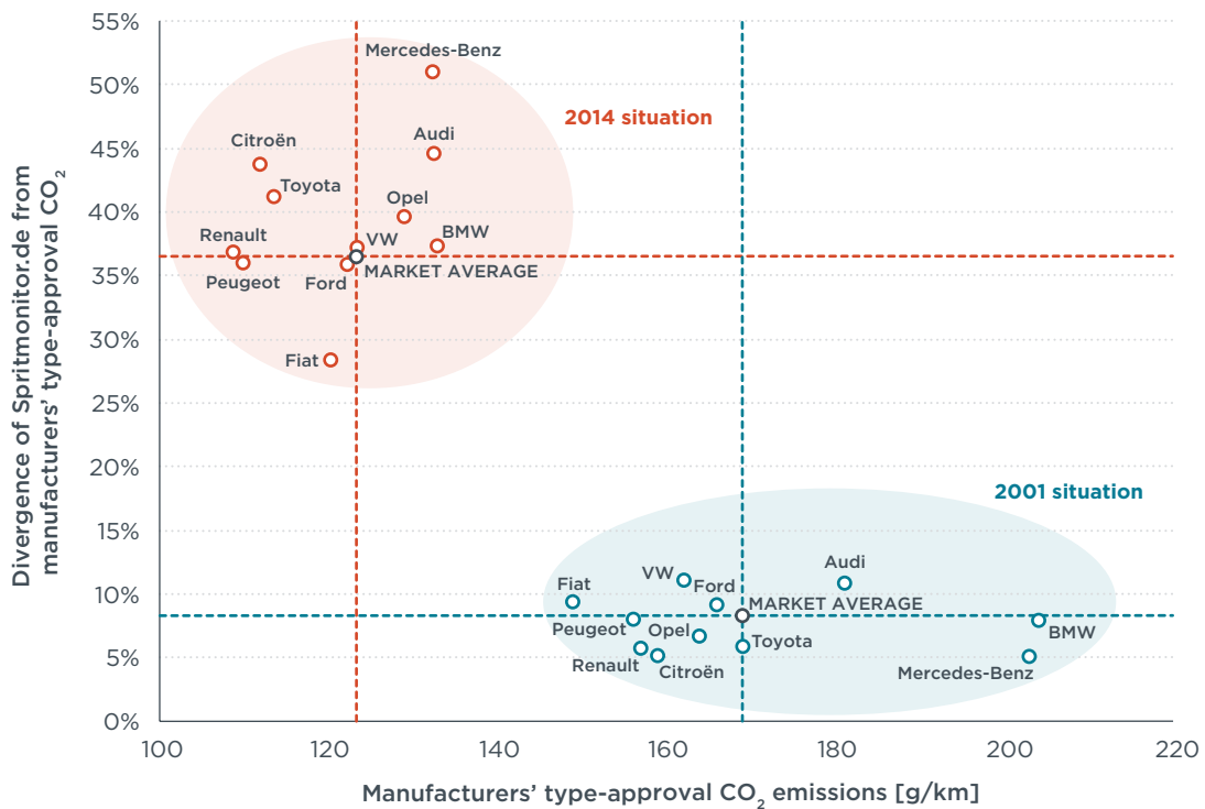
Figure 32. Type-approval CO 2 emission values and the corresponding divergence from Spiritmonitor.de for selected brands/manufacturers in 2001 and 2014.
