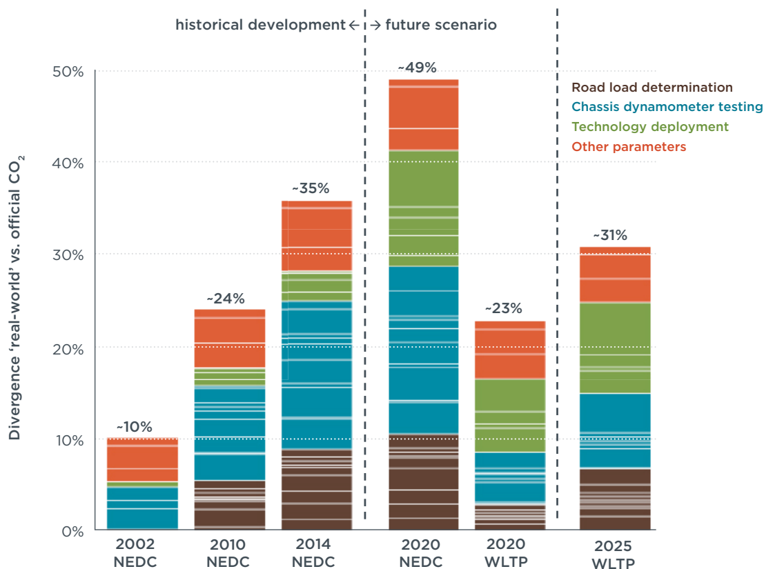
Figure 29: Estimate of the reasons for the divergence between type-approval and real-world CO 2 emission levels for new passenger cars in the past as well as in the future, with and without introduction of the WLTP (for details, see Stewart, Hope-Morley, Mock, & Tietge, 2015).
