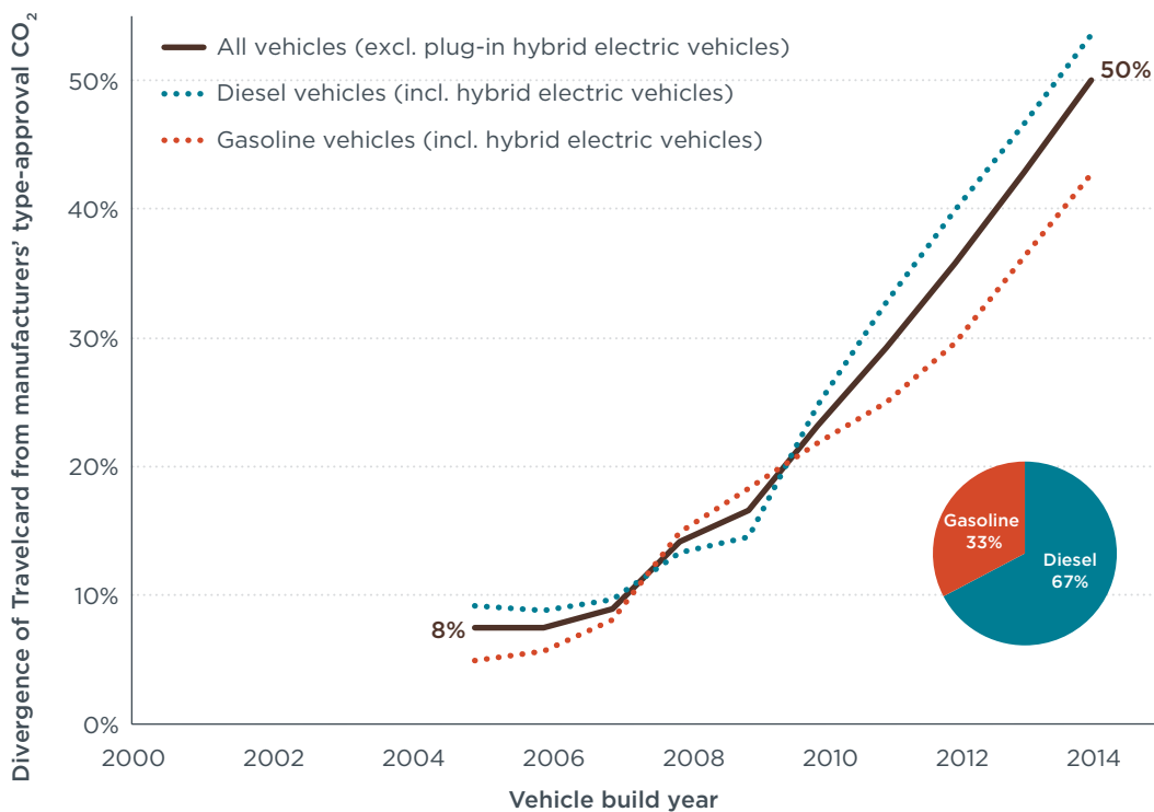
Figure 11. Divergence of Travelcard data from manufacturers' type-approval CO 2 emissions by fuel type (pie chart indicates share of vehicles per fuel type in the data set for 2014).
