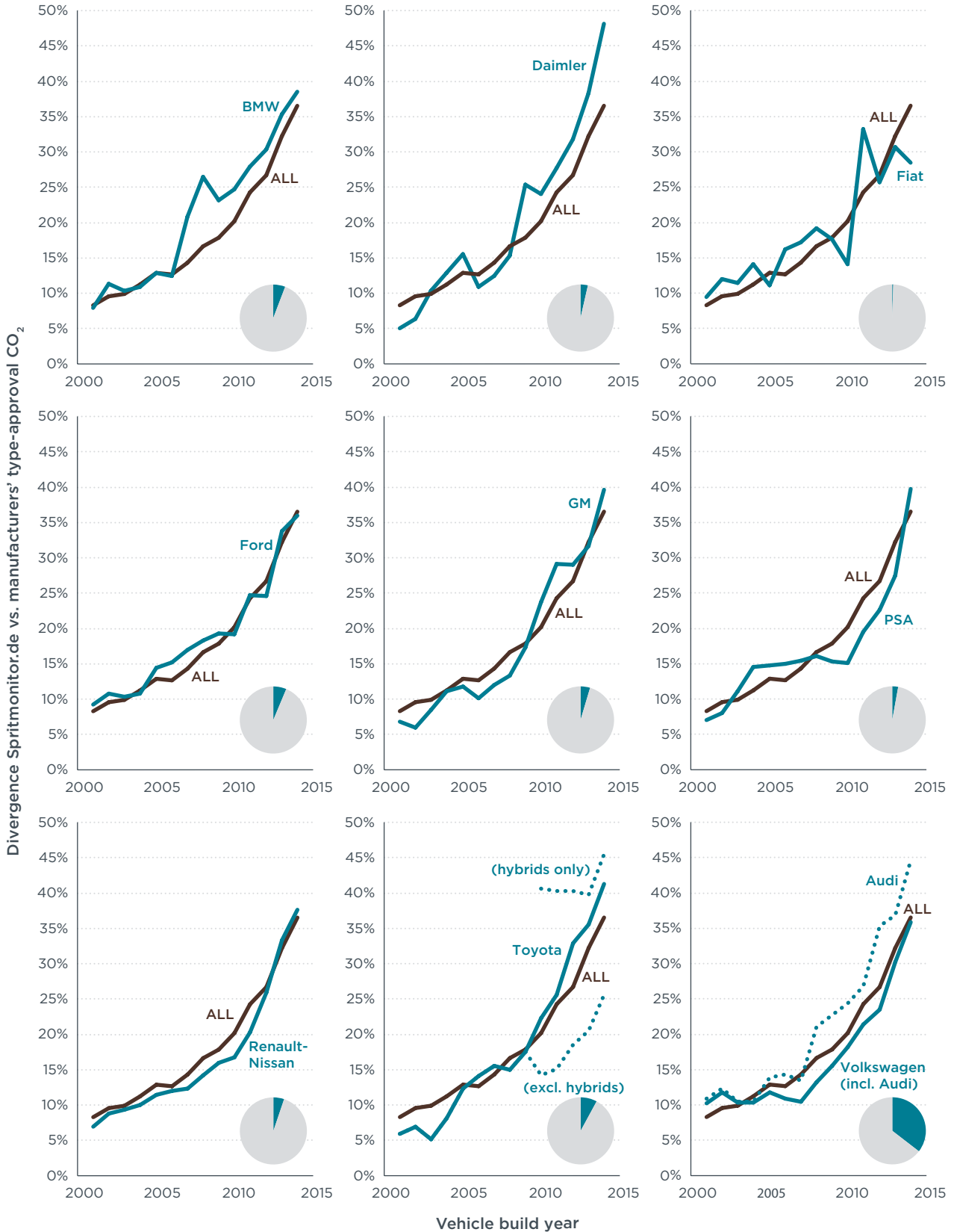
Figure 8. Divergence of Spritmonitor.de from manufacturers' type-approval CO 2 emissions by brands/manufacturers (pie chart represents the share of vehicles per manufacturer in the data set for 2014) 11 .
