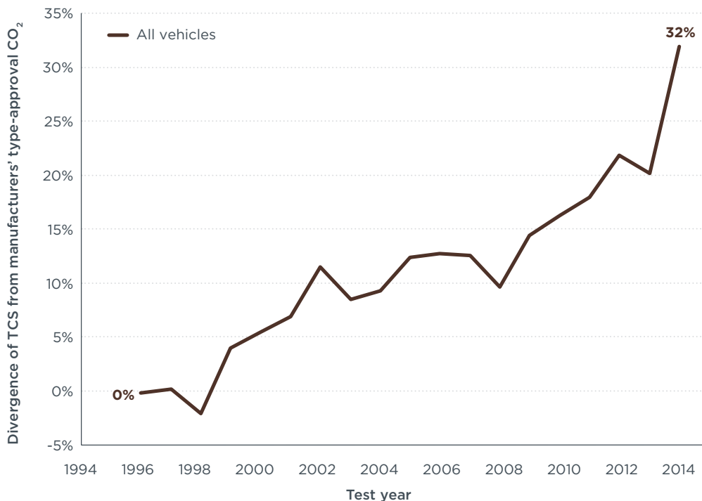
Figure 24. Divergence of TCS data from manufacturers’ type-approval CO 2 values.
