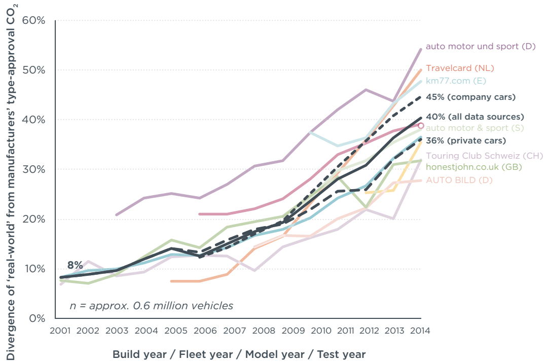
Figure 26. Divergence between real-world and manufacturers' type-approval CO 2 emissions for various real-world data sources, including average estimates for private cars, company cars, and all data sources.
