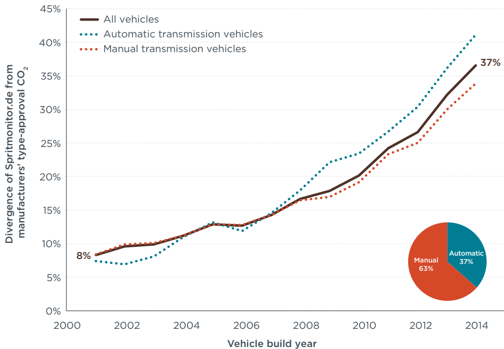
Figure 6. Divergence of Spritmonitor.de from manufacturers' type-approval CO 2 emissions by transmission type (pie chart indicates the share of vehicles per transmission type in the data set for 2014).
