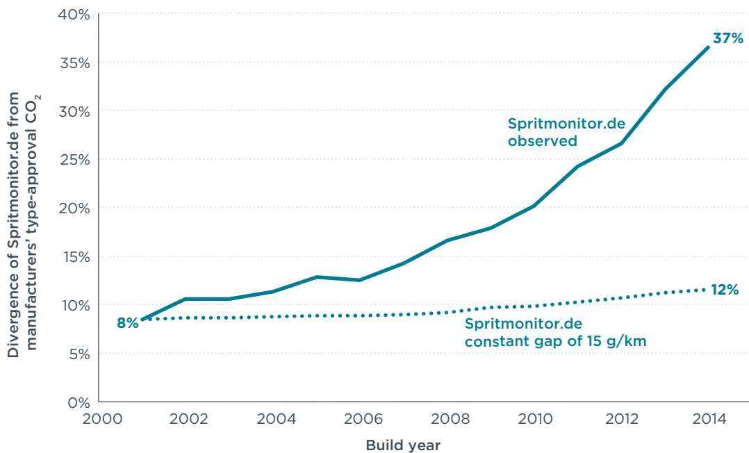
Figure 27. Divergence observed in Spritmonitor.de data compared with a hypothetical scenario where the divergence remained constant in absolute terms (15 g/km).
