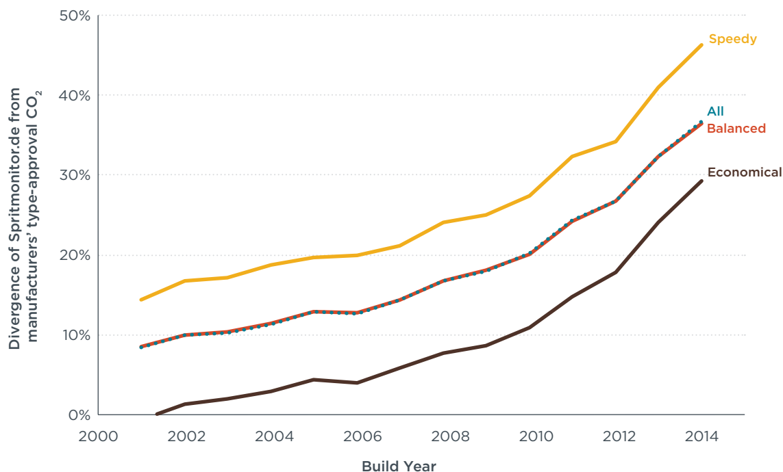
Figure 28. Divergence between Spritmonitor.de and type-approval CO 2 values for different driving styles, including economical , balanced , and speedy driving.
