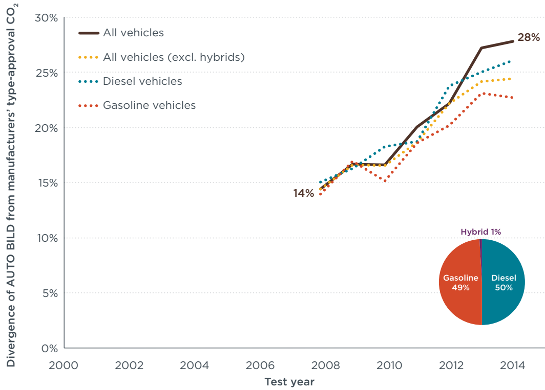
Figure 19. Divergence of AUTO BILD data from manufacturers' type-approval CO 2 emissions by fuel type (pie chart indicates the share of vehicles per fuel type in the data set for 2014).
