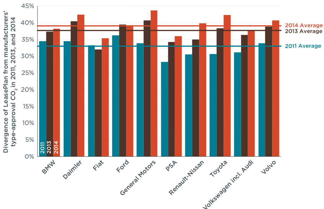
Figure 15. Divergence of LeasePlan data from manufacturers' type-approval CO 2 emissions by manufacturer/brand for 2011, 2013, and 2014. 24
