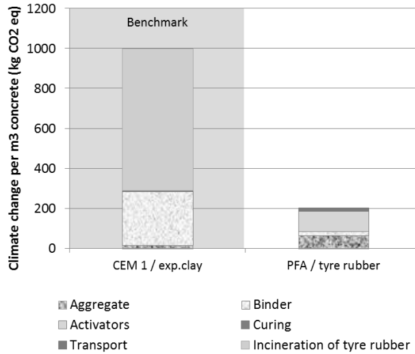
Figure 6: Carbon footprint of 1 m 3 of concrete blocks: influence of avoided end-of-life treatment (burden of waste treatment added to greenhouse gas emissions of benchmark concrete)
