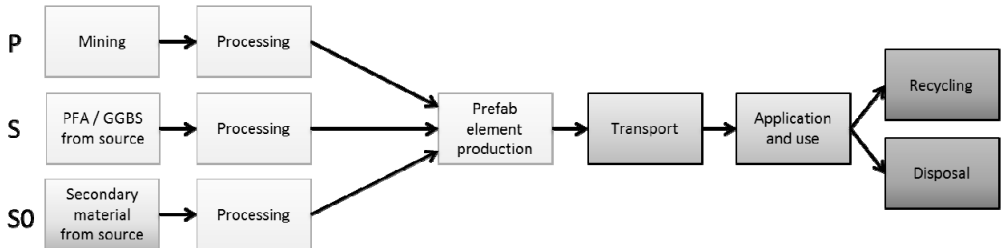
Figure 1: Scope of assessment for innovative concrete. P=primary raw materials, S=secondary materials, S0=secondary raw materials with few alternative destinations
