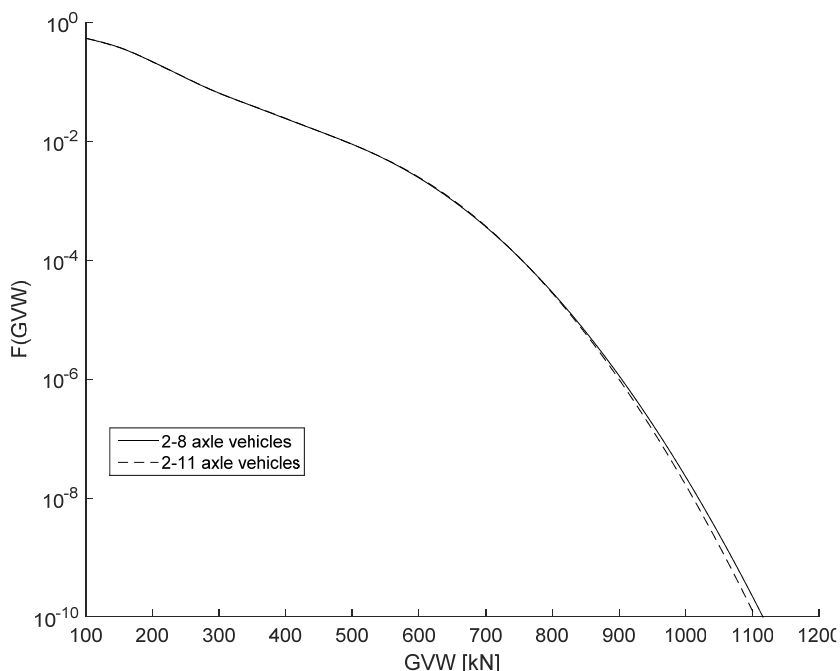
Figure 3. Exceedance probability of GVW based on statistical distribution of all measurements
