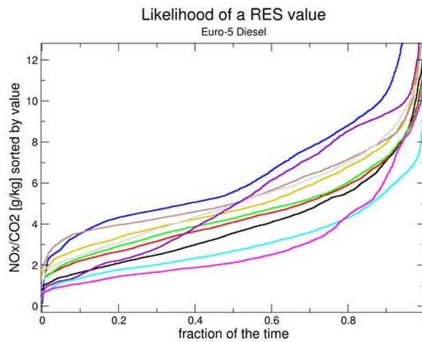
Figure 2 The sorted specific \text{NO}_x , or \text{NO}_x per \text{CO}_2 emissions, on the CADC test in the laboratory for different Euro-5 diesel vehicles. Only in a short part of the test the emissions are extremely high. The area under the curve is a measure of the total, or average, emission.
