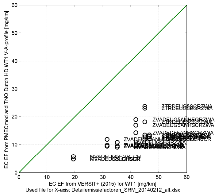
Figure 16 New EC emission factors for road type WT1 (urban) compared to those from current emission factor list.
