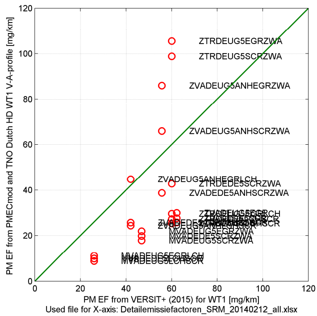
Figure 15 New PM emission factors for road type WT 1 (urban) compared to those from current emission factor list.
