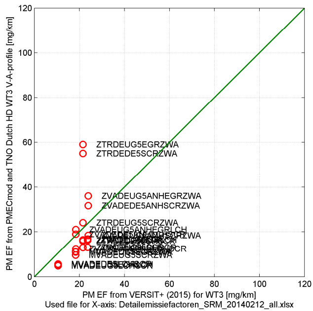
Figure 19 New PM emission factors for road type WT3 (motorway) compared to those from current emission factor list.
