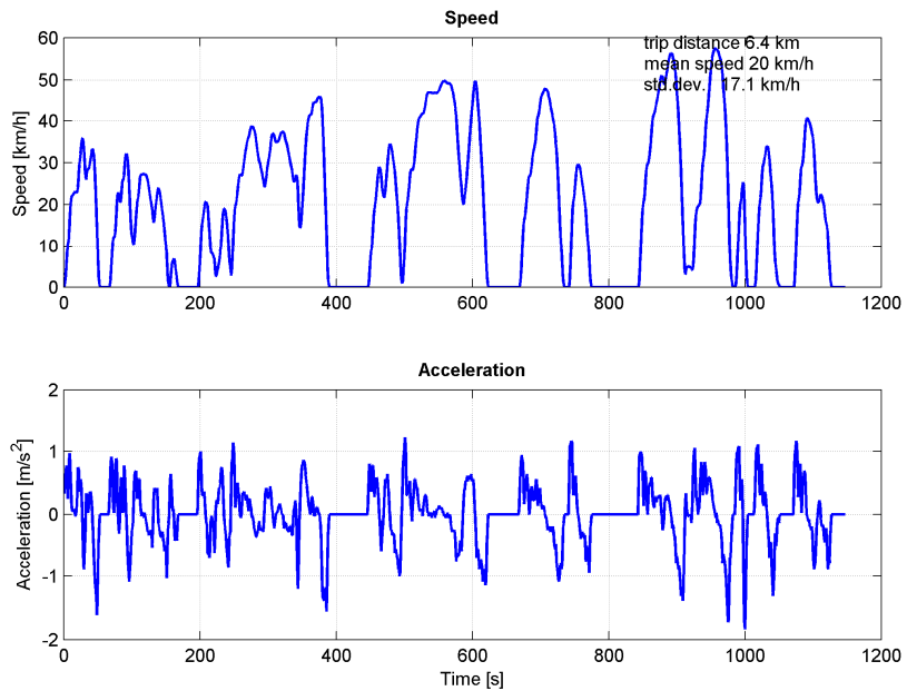
TNO Dutch HD V-A-profiles, Truck, Urban (WT1)
