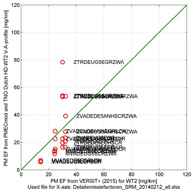
Figure 17 New PM emission factors road type WT2 (rural) compared to those from current SRM emission factor list.
