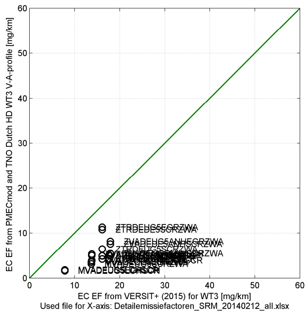
Figure 20 New EC emission factors for road type WT3 (motorway) compared to those from current emission factor list.
