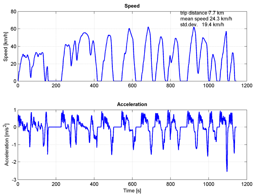
TNO Dutch HD V-A-profiles, Truck with trailer, Urban (WT1)
