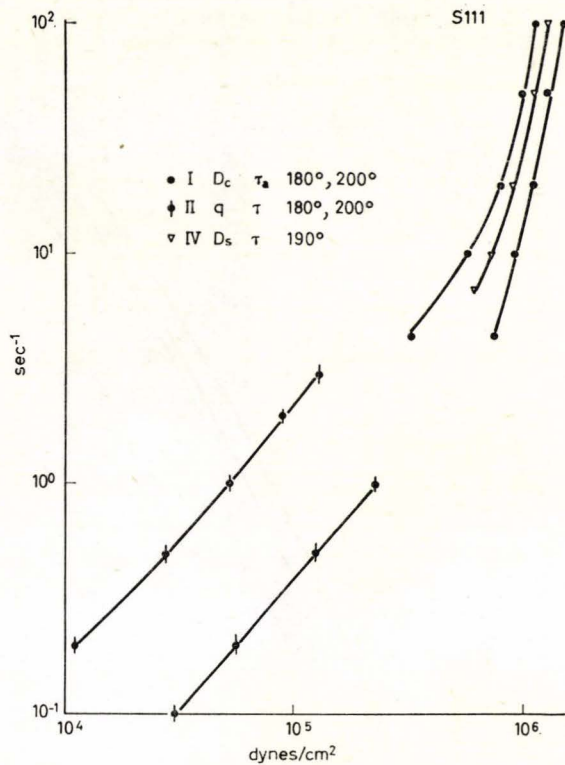
Figure 1 a. Results obtained for S 111 without application of Rabinowitch corrections.
