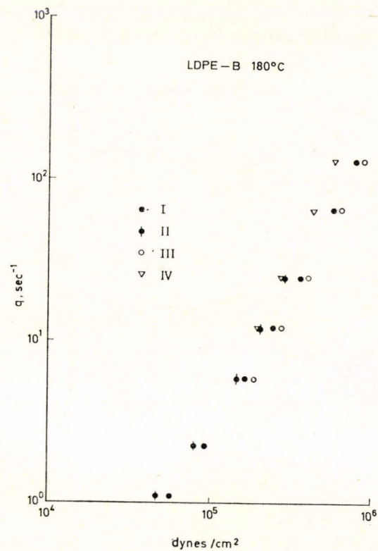
Figure 2 d. Results obtained for LDPE-B with Rabinowitch corrections.
