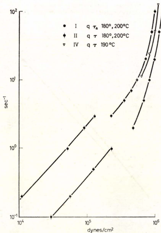
Figure 2 a. Results obtained for S 111 with Rabinowitch corrections.
