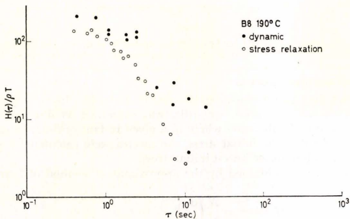
Figure 9 b. The relaxation spectra for B 8 as obtained from the dynamic moduli by the method of Ninomiya and Ferry and from stress relaxation by the method of Ferry and Williams.
