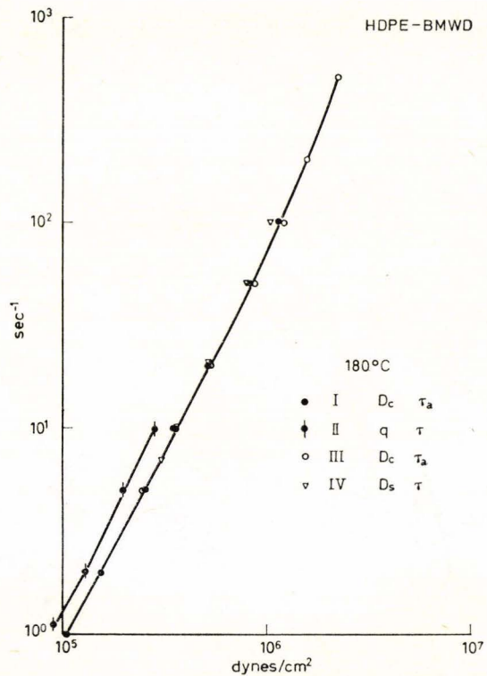
Figure 1 f. Results obtained for HDPE-BMWD without application of Rabinowitch corrections.
