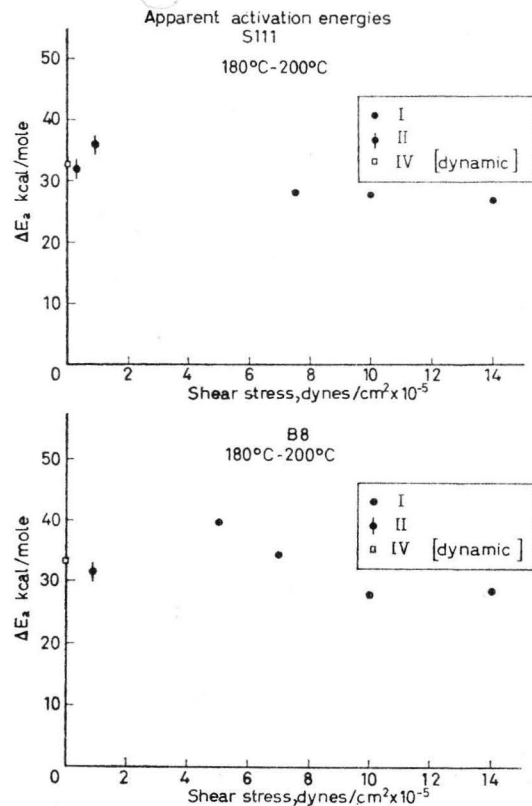
Figure 4 a. Apparent energies of activation for polystyrenes as function of the shear stress from steady shear flow measurements.
