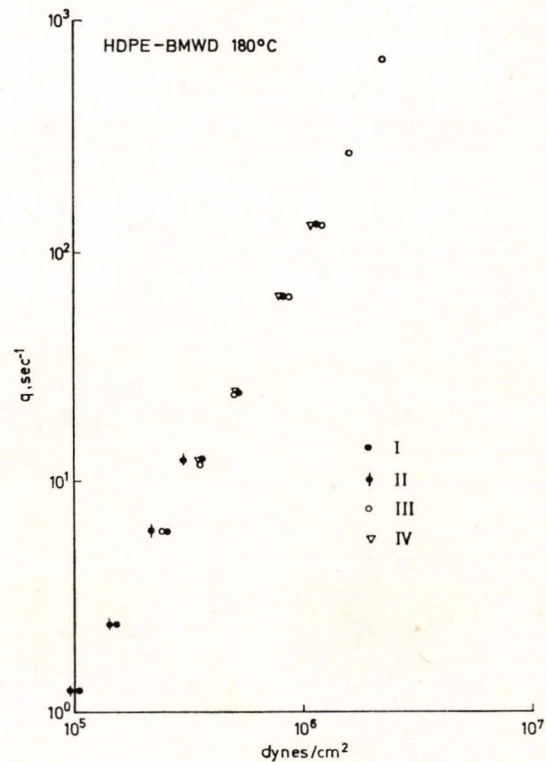
Figure 2f. Results obtained for HDPE-BMWD with Rabinowitch corrections.
