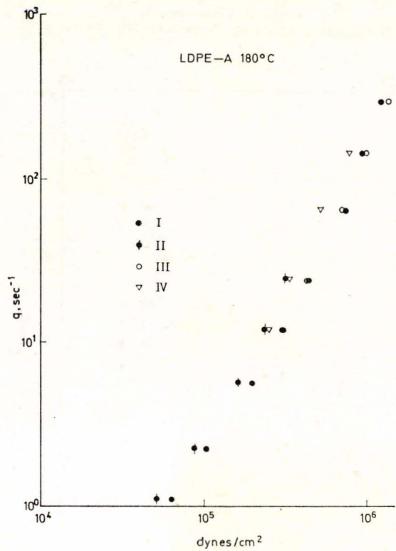
Figure 2 c. Results obtained for LDPE-A with Rabinowitch corrections.
