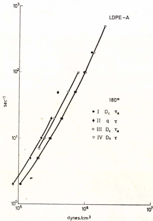
Figure 1 c. Results obtained for LDPE-A without application of Rabinowitch corrections.
