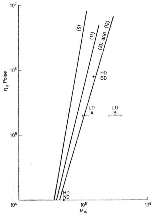
Figure 3. Newtonian viscosities at 150°C for the polyethylenes compared with data from literature.
