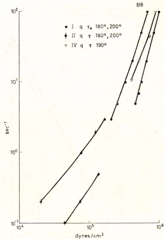
Figure 2 b. Results obtained for B 8 with Rabinowitch corrections.
