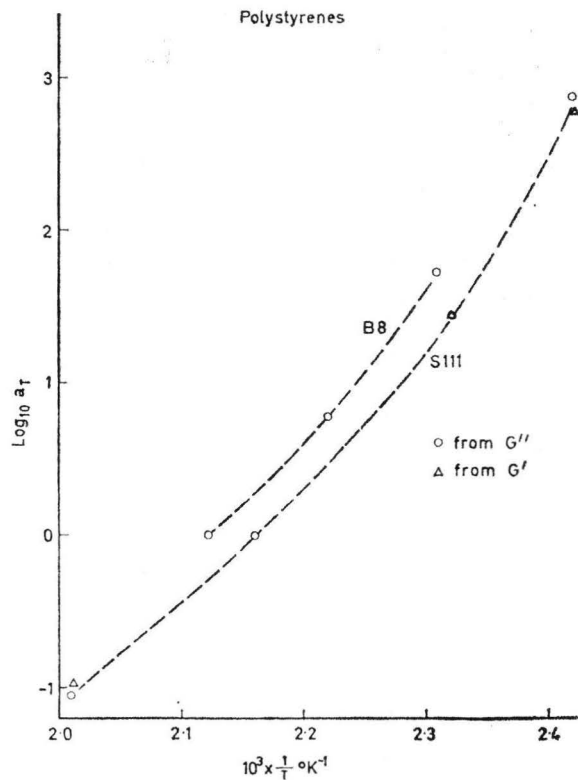
Figure 5 a. Shift factor a_T for the polystyrenes as used by IV in the dynamic viscosity measurements.
