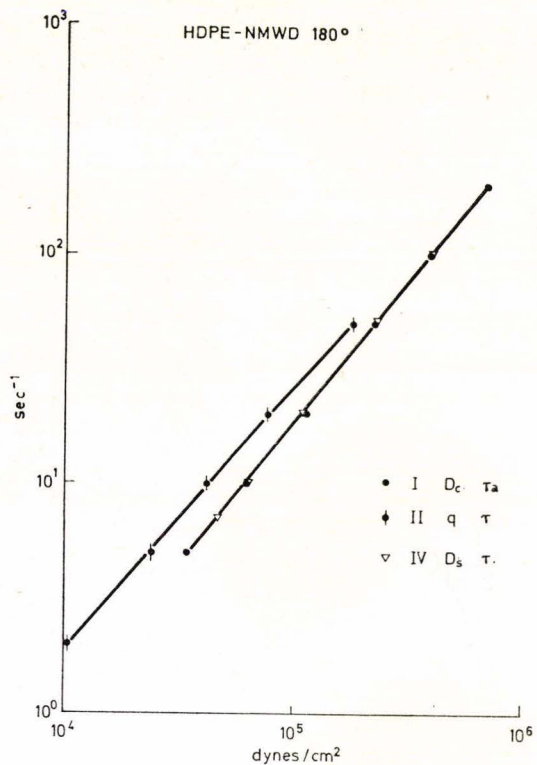
Figure 1 e. Results obtained for HDPE-NMWD without application of Rabinowitch corrections.
