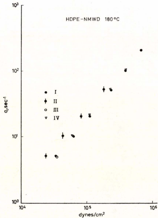
Figure 2e. Results obtained for HDPE-NMWD with Rabinowitch corrections.
