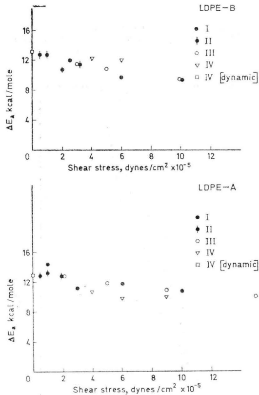
Figure 4 b. Apparent energies of activation for low density polyethylenes as function of the shear stress from steady shear flow measurements.
