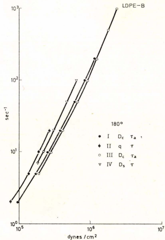
Figure 1 d. Results obtained for LDPE-B without application of Rabinowitch corrections.
