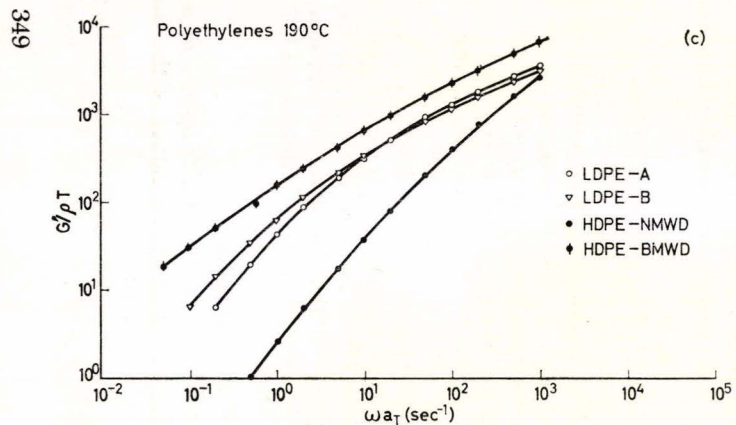
Figure 6. (a) The reduced modulus G'/\rho T as function of frequency for the polystyrenes. (b) The reduced modulus G''/\rho T as function of frequency for the polystyrenes. (c) The reduced modulus G'/\rho T as function of frequency for the polyethylenes. (d) The reduced modulus G''/\rho T as function of frequency for the polyethylenes.
