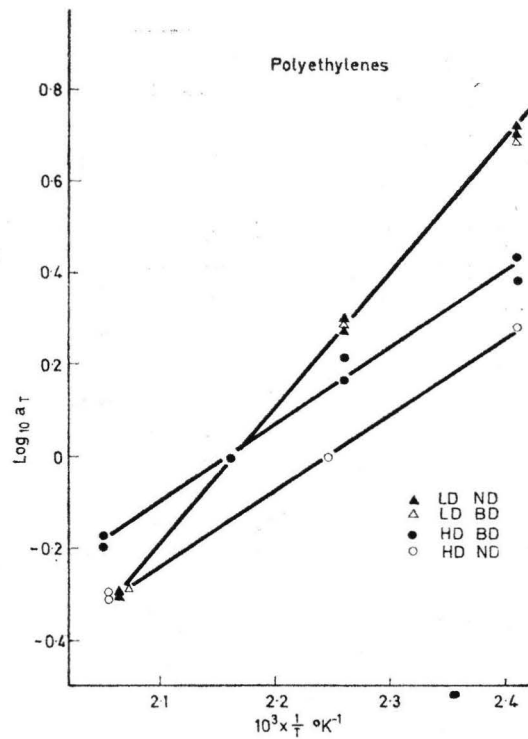
Figure 5 b. Shift factor a_T for the polyethylenes as used by IV in the dynamic viscosity measurements.
