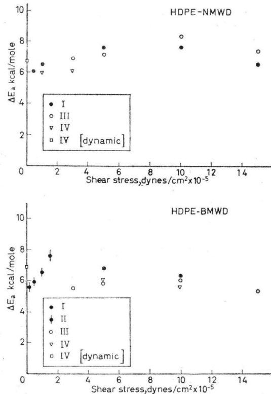
Figure 4 c. Apparent energies of activation for high density polyethylenes as function of the shear stress from steady shear flow measurements.
