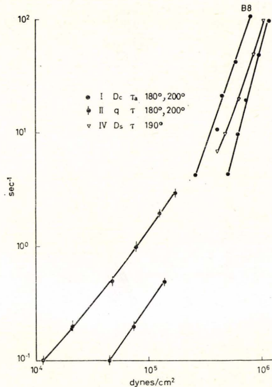
Figure 1 b. Results obtained for B 8 without application of Rabinowitch corrections.
