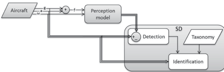
Figure 5. Flow of automatic detection and identification of SD events from the flight data recorder.
