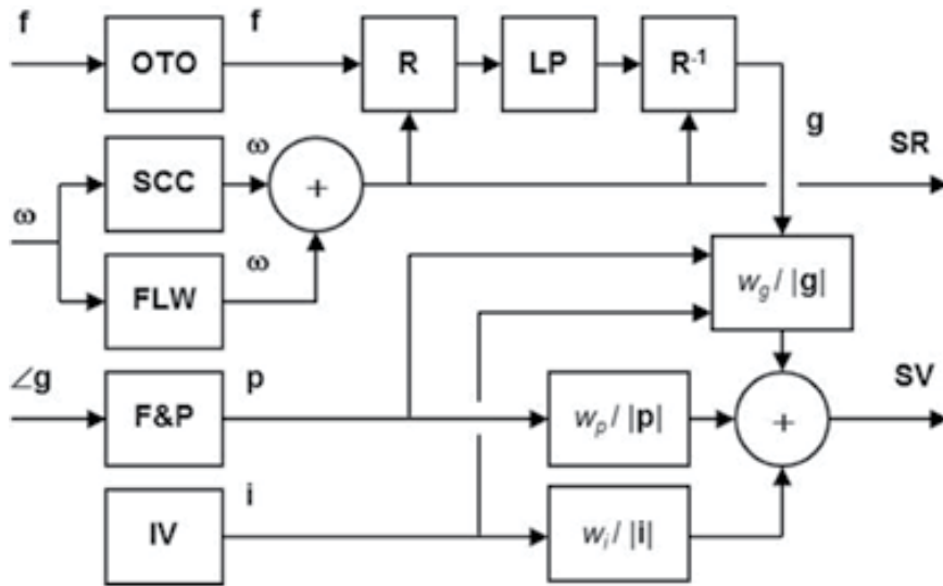
Figure 2. Outline of TNO perception model showing the neural mechanism to resolve the perceptual ambiguity in the sensed specific force f into the subjective vertical (SV) Legend: OTO=otoliths; SCC=semicircular canals; FLW=optic flow; F&P=visual frame and polarity; IV=idiotropic vector ( i ); R=rotation matrix, LP = low-pass filter.
