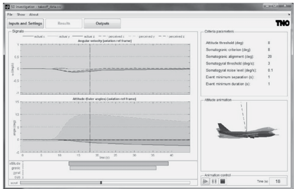
Figure 7. Example of model output during takeoff. The bottom tracks "attitude" and "grav" indicate the somatogravic illusion.
