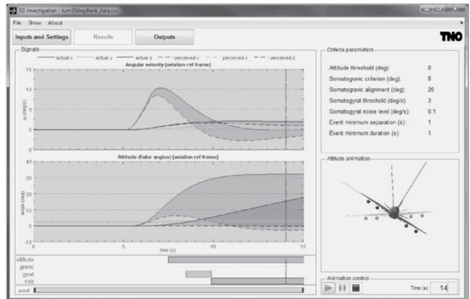
Figure 6. Screenshot of the model output during analysis of a coordinated turn. The bottom tracks “attitude,” “gyral,” and “sub” indicate that the maneuver induces a misperception of attitude, a somatogyral illusion, and also contains an episode of sub-threshold motion.
