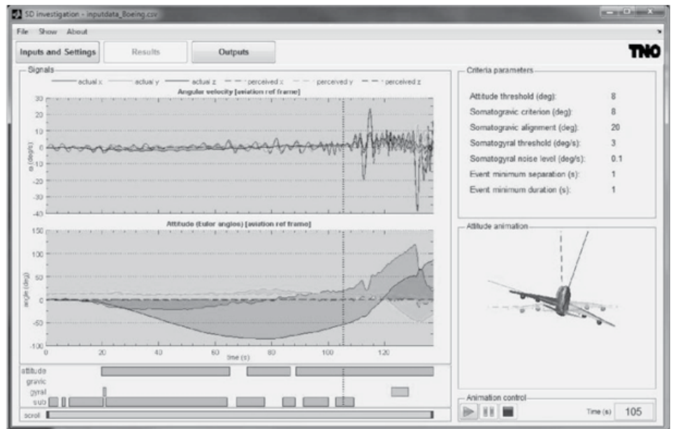
Figure 8. Model analysis of a B-737 LOC accident showing 140 s of actual and perceived angular motion (upper time history) and actual and perceived roll and pitch attitude (lower time history). The SD tracks indicate issues with perceived attitude as well as sub-threshold angular motion through the larger part of recorded flight.
