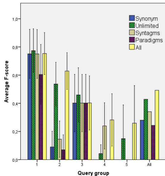
Graph 6. F-score Image Retrieval for High Effectiveness.
