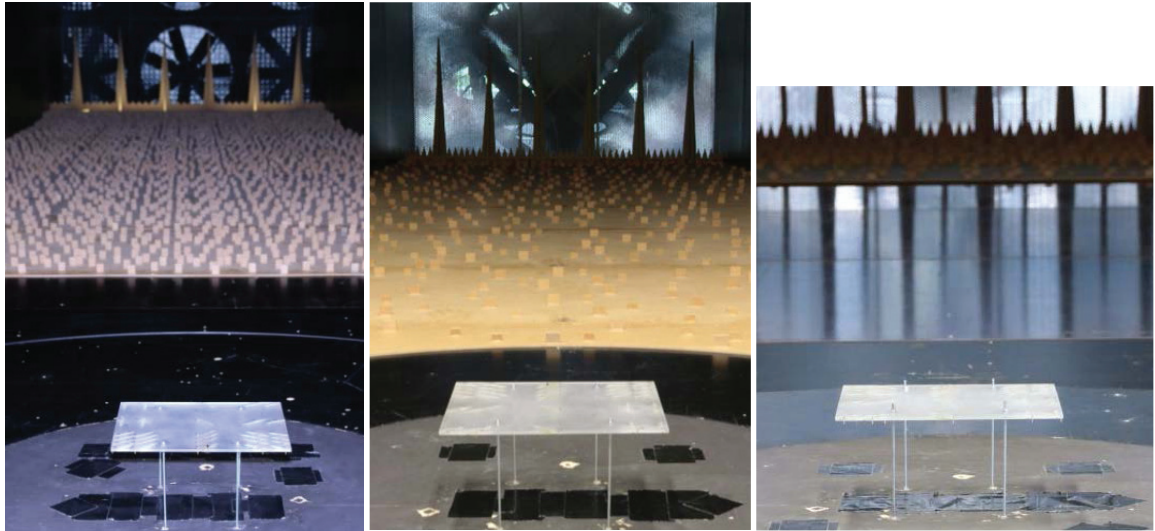
Fig. 6. Spires, fence and roughness elements in wind tunnel to generate boundary layer of 21% (BL1, left), 18% (BL2, middle) and 13% (BL3, right) longitudinal turbulence intensity in height of the heliostat.
