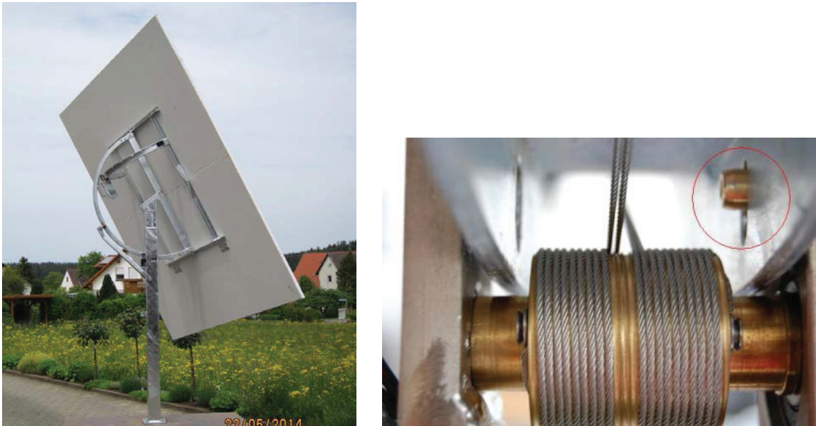
Fig. 1.: Left: First rim drive prototype with 8 m 2 mirror surface (photo by SOLTEC); Right: Winch wheel cable drive system, locking position of the smaller rim drive. The red circuit shows the extended adjust pin.
