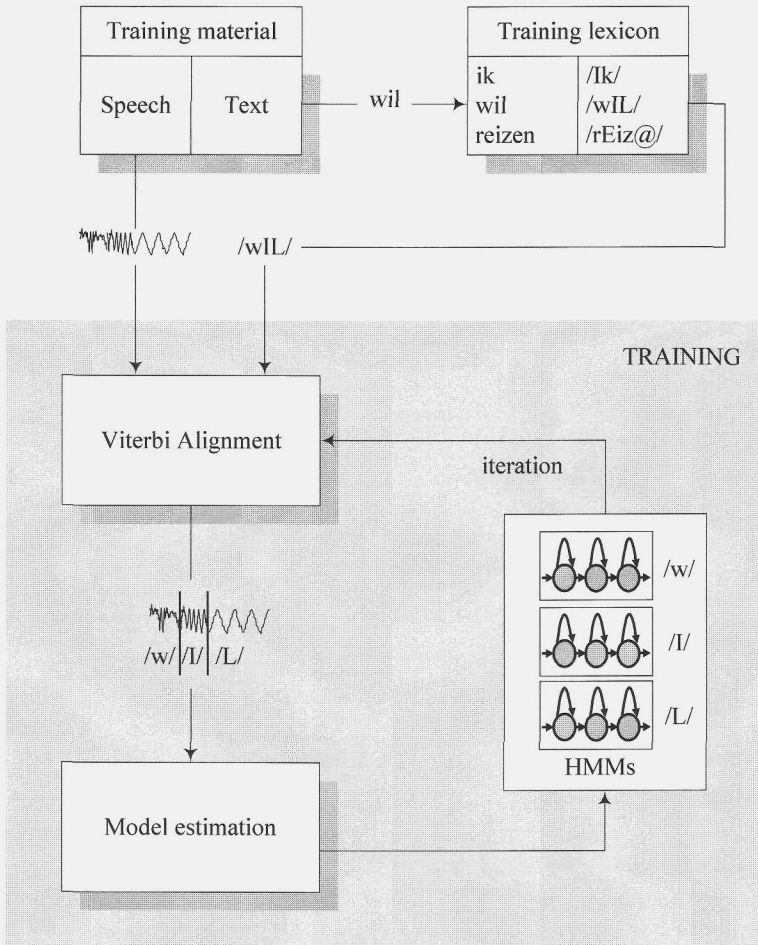
Figure 3: Training the acoustic models
