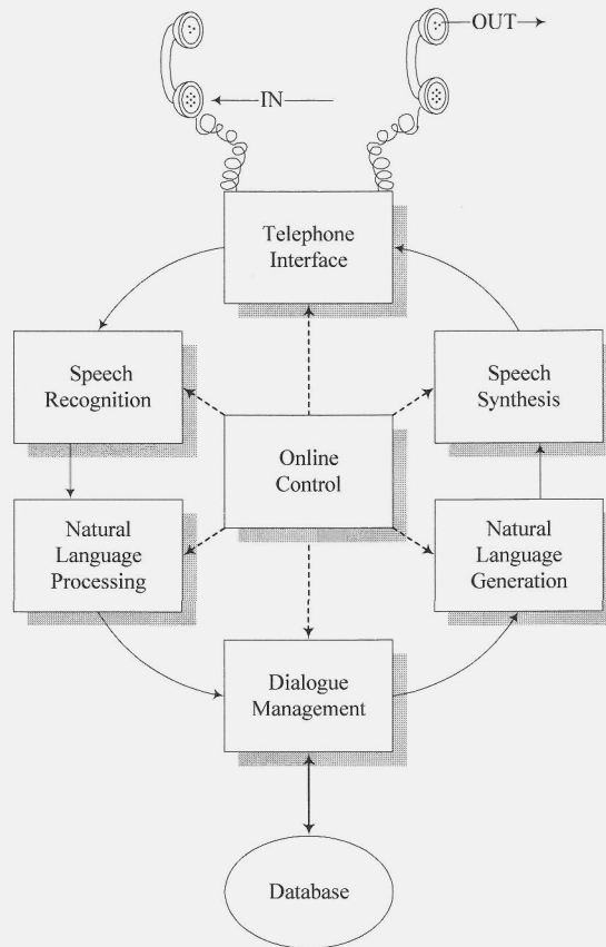
Figure 1: Architecture of the OVIS Spoken Dialogue System
