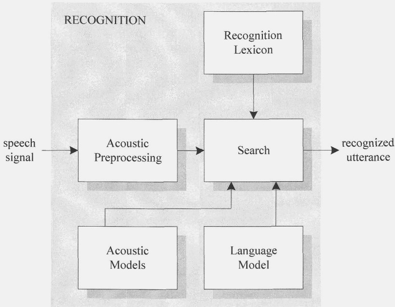
Figure 4: Recognition process
