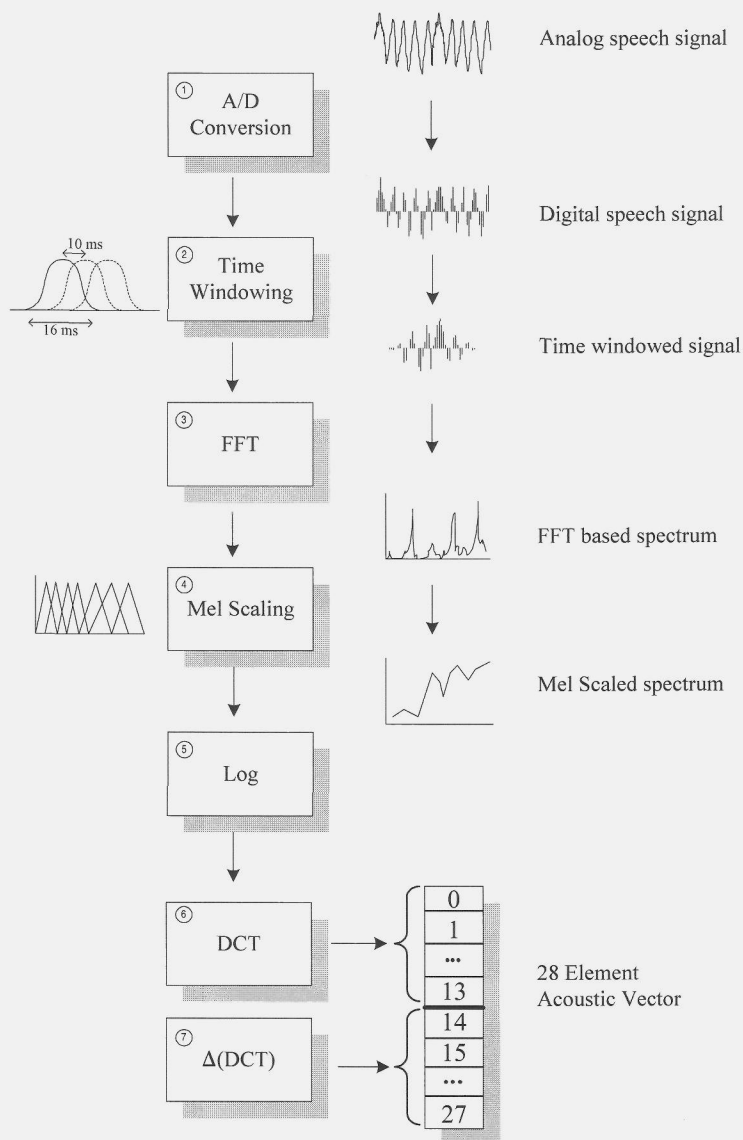
Figure 2: Acoustic pre-processing for obtaining MFCC-based feature vectors.
