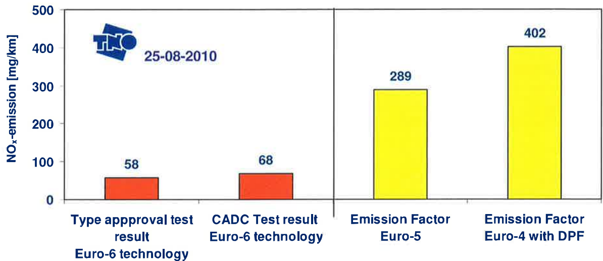
Figure 1: average NO x -emission during the type approval cycle and the cycle that represents European real World conditions (CADC), compared with the traffic emission factors [8] for Euro-5 and Euro-4 passenger cars with a diesel engine and particulate filter
