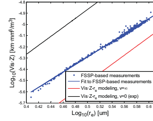
Fig. 11. Observations and modeling of Vis \cdot Z - r_e relation.
