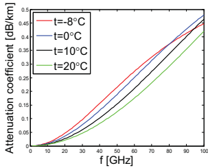
Fig. 5. Attenuation coefficient with LWC of 0.1 g/cm^3 .
