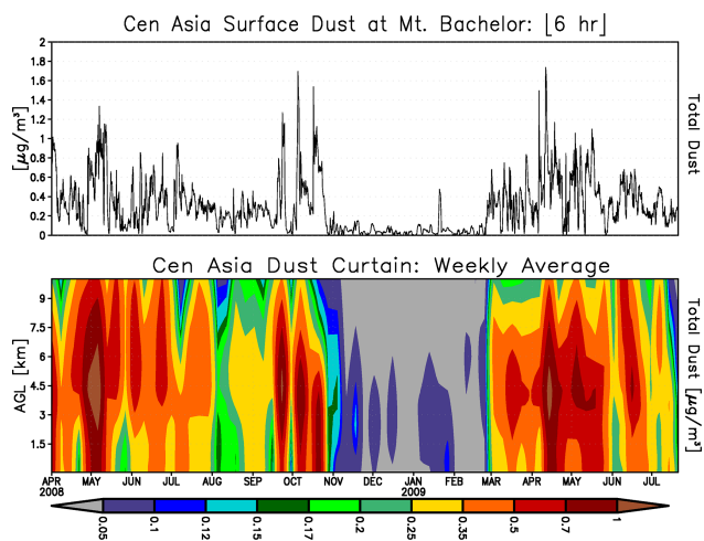
Figure 18. Time series of predicted surface concentration at 6 h time step (top panel) and weekly averaged time–altitude cross sections (bottom panel) of total dust (PM 10 ) from Central Asia dust emissions at Mt. Bachelor, Oregon, USA.
