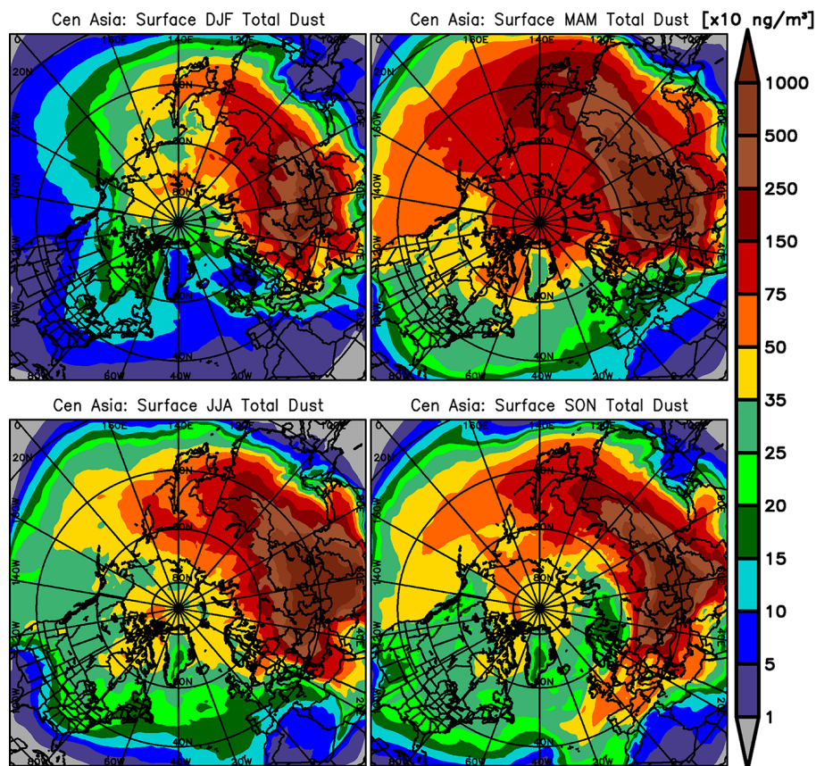
Figure 17. Seasonally averaged surface total dust (PM 10 ) concentrations from Central Asian dust emissions. DJF (top left panel) denotes the average for the months of December, January, and February. MAM (top right panel) denotes the average for months of March, April, and May. JJA (bottom left panel) denotes the average for months of June, July, and August. SON (bottom right panel) denotes average for months of September, October, and November.
