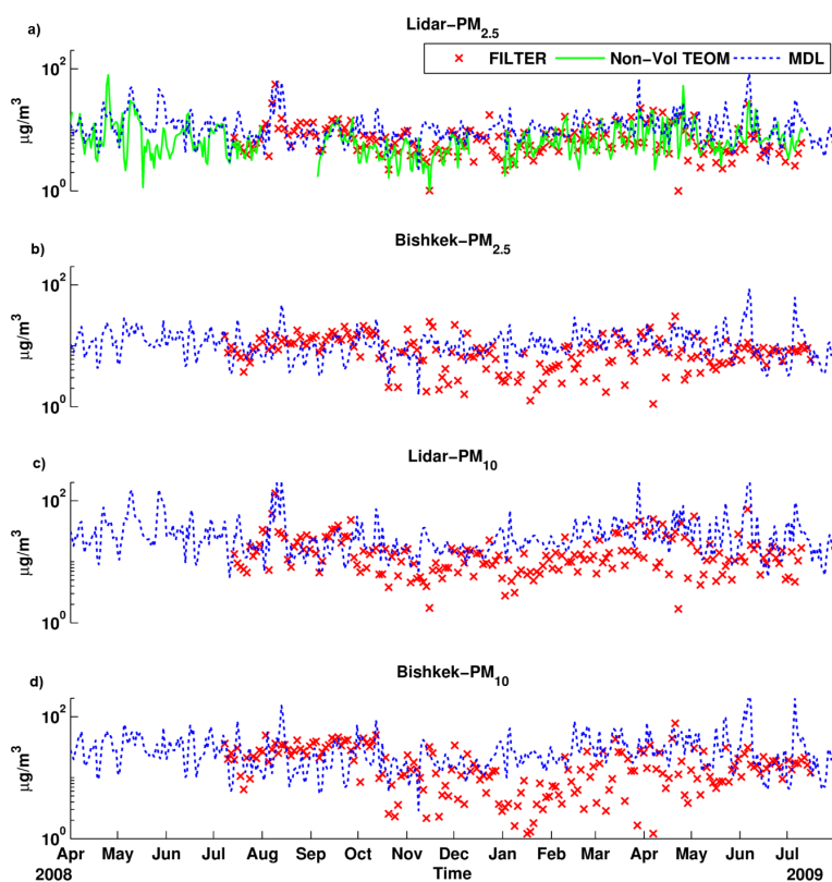
Figure 9. Comparison of simulated PM mass with filter-based observations at Central Asian sites. (a) PM 2.5 (LST) along with TEOM non-volatile measurements, (b) PM 2.5 (Bishkek), (c) PM 10 (LST), and (d) PM 10 (Bishkek) in ( \mu\text{g m}^{-3} ). “Lidar” denotes the LST site.
