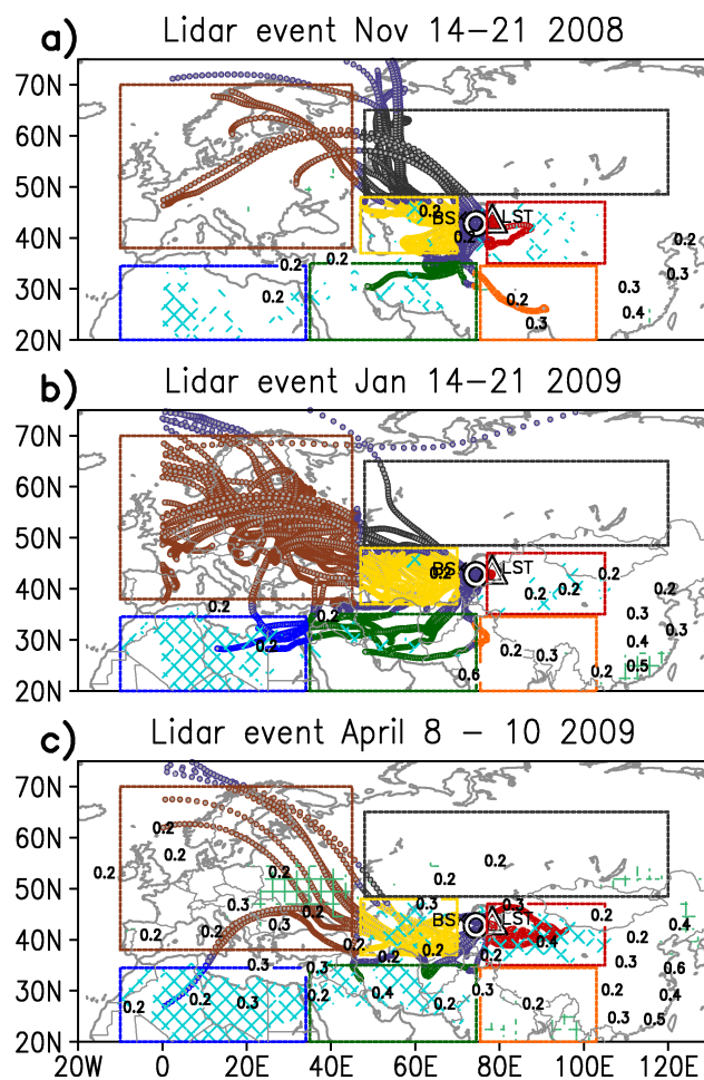
Figure 15. Same as Fig. 14 but for November 2008, January 2009, and April 2009 (events 3, 4, and 5 denoted in Fig. 13).
