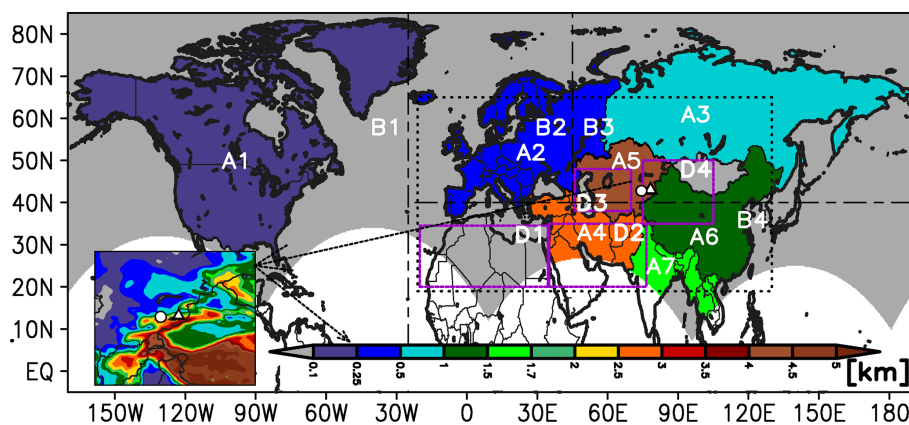
Figure 1. WRF-STEM modeling domain setup and source region definition used in the simulations. Modeling analysis was done on the hemispheric scale. The black dotted rectangular box denotes the subset of the modeling domain used in this analysis. The triangle and circle markers denote locations of the Lidar Station Teplokluchenka (LST) and Bishkek observation sites. The anthropogenic source regions are denoted by colored regions with the A notation: A1 (North America), A2 (Europe), A3 (Russia), A4 (Middle East), A5 (Central Asia), A6 (China), and A7 (South + Southeast Asia). The dust source regions are indicated by the magenta rectangles with the D notations: D1 (Africa), D2 (Middle East), D3 (Central Asia), and D4 (western China). The biomass burning sources regional boundaries are indicated by the long dashed black lines with B notations: B1 (North America, i.e., region west of 25° W), B2 (Europe, i.e., region west of 45° E and 40° N and above), B3 (Siberia: i.e east of 45° E and 40° N and above), and B4 (South Asia, i.e., below 40° N). The insert shows the topography around the observation sites.
