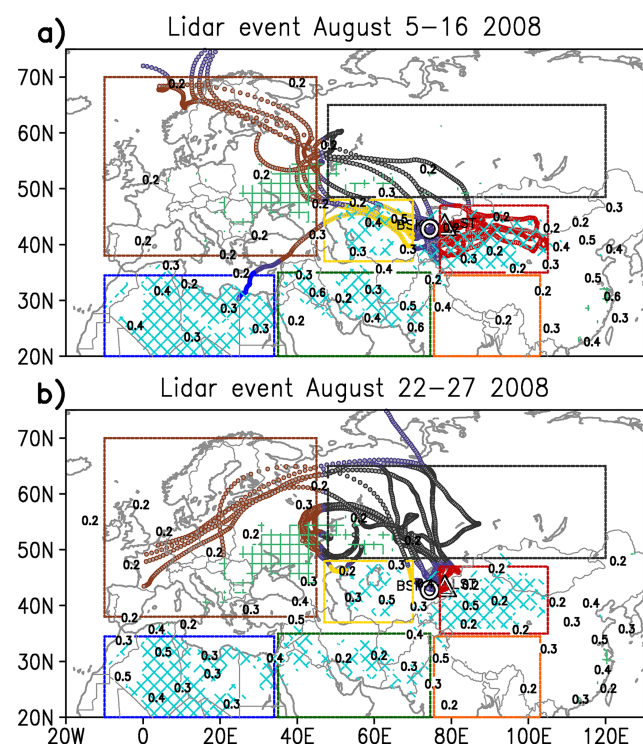
Figure 14. Ten-day air mass back trajectories for August 2008 (events 1 and 2 as denoted in Fig. 13) color-coded by source regions. The blue diamond and green square hatched areas denote the natural dust and biomass burning emission sources, while the numbers in black denote MODIS AOD contours averaged over the event time period and prior 10 days. The trajectories are color-coded by source regions: Africa (blue), Middle East (green), Central Asia (yellow), North Asian biomass ( >50^{\circ} N, black), Europe (brown), China (red), and South Asia (orange). “Lidar” denotes the LST site.
