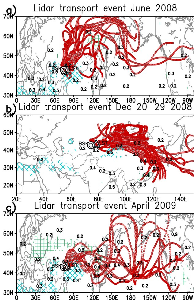
Figure 16. Ten-day air mass forward trajectories illustrating the seasonality in transport pathways out of CA for (a) June 2008, (b) December 2008, and (c) April 2009. The blue diamond and green square hatched areas denote the natural dust and biomass burning emission sources, respectively, while the numbers in black denote MODIS AOD contours averaged over the event time period and subsequent 10-day time window. “Lidar” denotes the LST site.
