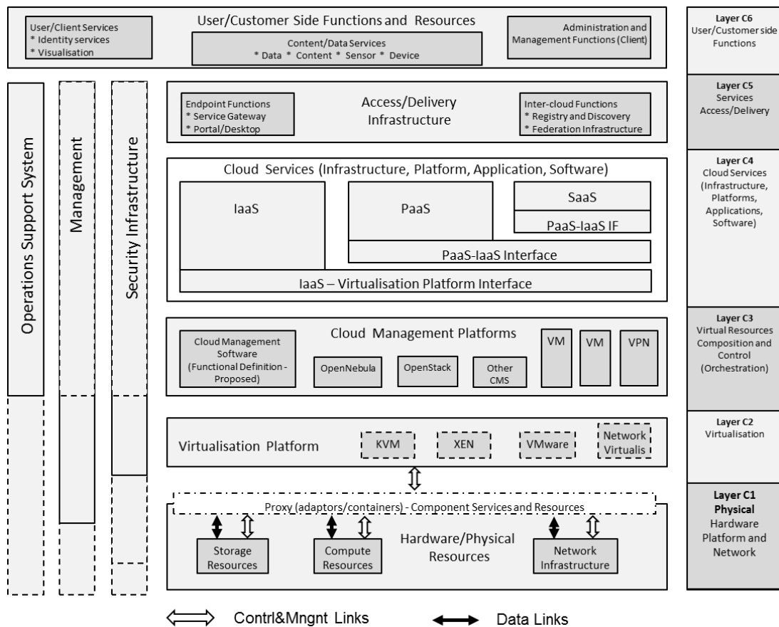
Figure 2.4. Reference Multilayer Cloud Services Model (CSM).
