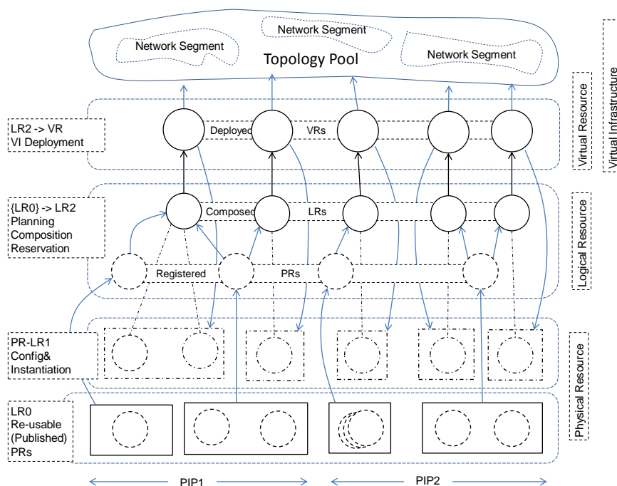
Figure 16. Relation between different resource presentations in relation to different provisioning stages.
