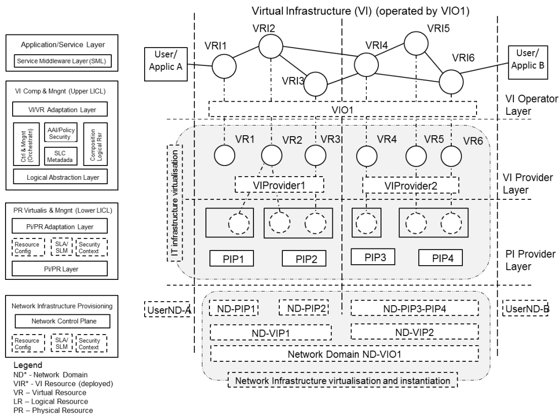
Figure 14. Main actors, functional layers and processes in on-demand infrastructure services provisioning
