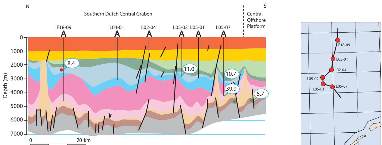
Fig. 11. N-S cross-section through southern Dutch Central Graben, showing the distribution of observed fluid overpressures and its relation with the hydrogeological framework. For legend see Fig. 10.
