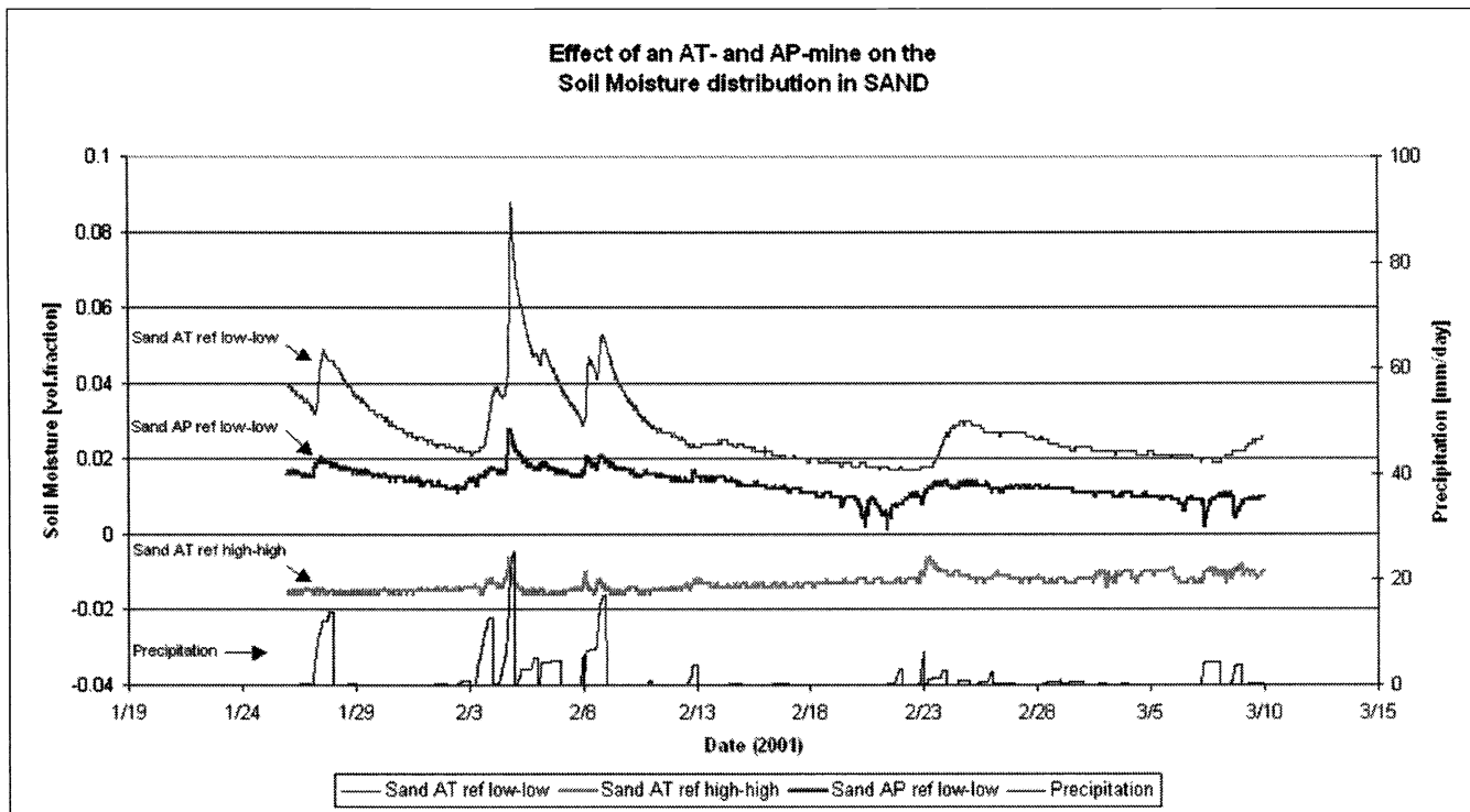
Figure 6. Effect of an AT and AP-mine on the soil water distribution in sand.
