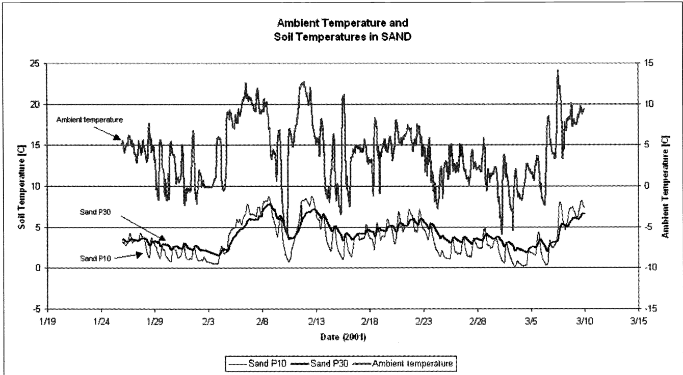
Figure 8. Ambient and soil temperatures in sand test lane (P10, P30 at depth 10 and 30 cm respectively).
