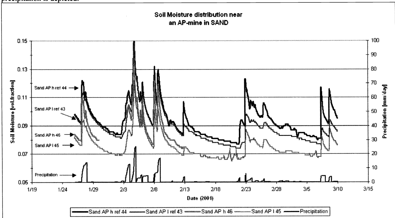
Figure 4. Soil water distribution around an AP-mine in sand.
