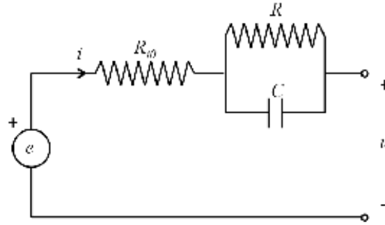
Figure A.10: RC circuit battery model.
