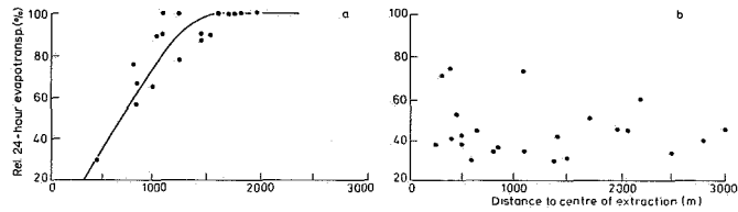
Figure 5 Relative 24 hour transpiration ( \lambda E_p^{24} / \lambda E_p^{24} ) on 30 July 1982 as a function of distance to the centre of the extraction. Data were derived from the transpiration map shown in Figure 4 for (a) grassland plots on Typic Haplaquod soil with a relatively shallow groundwater table and (b) maize plots on Typic Haplaquod soil with a relatively deep groundwater table. The mentioned groundwater tables apply to the situation without groundwater extraction
