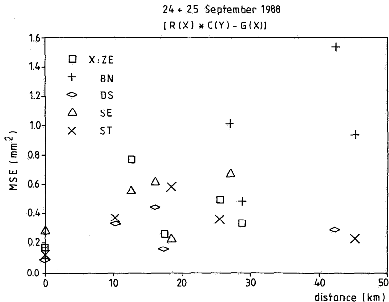
Figure 5 Mean square error ( \text{mm}^2 ) of the radar data calibrated by calibration factors of all five raingauge locations plotted as a function of distance between the locations (km)
