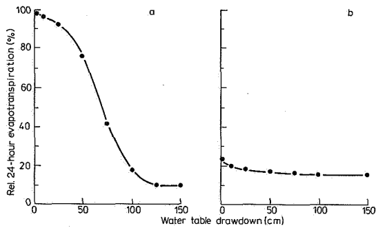
Figure 6 Relative 24 hour transpiration ( \lambda E_p^{24} / \lambda E_p^{24} ) on 30 July 1982 as a function of groundwater table drawdown, simulated with the model SWATRE for (a) grassland plots on Typic Haplaquod soil with a relatively shallow groundwater table and (b) maize plots on Typic Haplaquod soil with a relatively deep groundwater table. The mentioned groundwater tables apply to the situation without groundwater extraction
