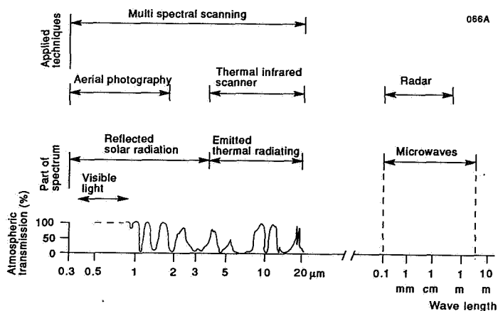
Figure 1 Overview of the electromagnetic spectrum, the transmission of the atmosphere for the different wave lengths and the applied remote sensing techniques
