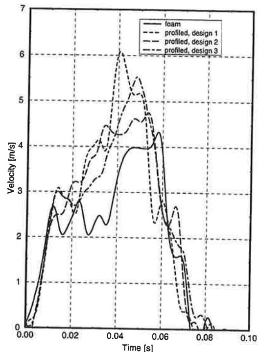
Figure 3: 'Door' velocities with four different barriers.
