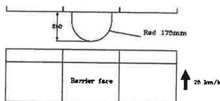
Figure 4. Central pole test.
