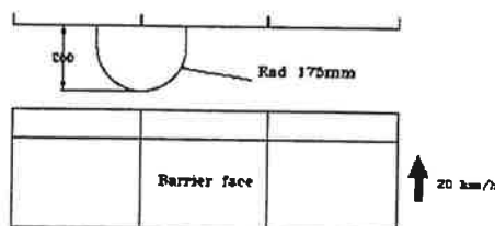
Figure 5. Offset Pole Test.
