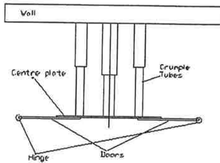
Figure 8. Yielding Wall Test.
