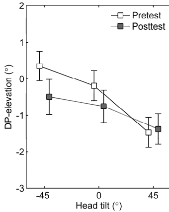
Figure 5.3: Mean DP-elevation as a function head tilt, averaged over the four centrifuge conditions (bars indicate standard error of mean). According the right-hand-rule, negative angles indicate backward tilt of the DP relative to the z-axis.
