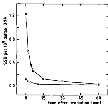
Fig. 3. Removal of SSB induced in normal human fibroblasts by irradiation with 110 \text{ kJ} \cdot \text{m}^{-2} UV-A during a subsequent incubation at 37^\circ\text{C} in a 5% \text{CO}_2 incubator (except the samples incubated for 2 and 4 min, which were placed on a wet brass plate with a temperature of 37^\circ\text{C} ). After the periods indicated in the figure, samples were used for the SSB determination. A single representative experiment is shown, performed in duplicate as in Fig. 2. \square , irradiation of cells in PBS; \circ , irradiation of cells in PBS with catalase.
