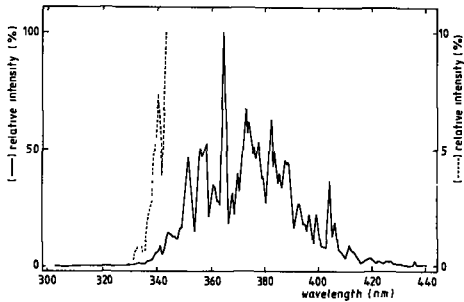
Fig. 1. The emission spectrum of the Sellas UV-A sunlamp type Sellasol 1200, filtered by an 8-mm thick plate of glass to eliminate light of wavelengths below 330 nm. The relative spectral energy distribution was measured through a Jarrel Ash monochromator operating at a bandwidth of 1.2 nm. Calibration was done by comparison with the radiant output of a HPK 125 Watt of Philips. In addition, the spectrum between 305 and 345 nm, recorded at a 10-fold higher sensitivity, has been plotted (-----).
