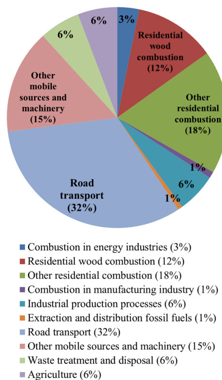
Fig. 8. Relative contribution from different source sectors to emissions of fine particulate elemental carbon ( EC_{2.5} ) in Europe in 2005, as estimated in the emission inventory developed within the EUCAARI project.
