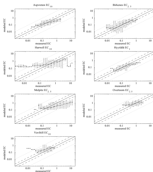
Fig. 4. Scatterplots of measured and modelled EC (standard model setup, STD) for seven European measurement stations: (a) Aspvreten EC 10 , (b) Birkenes EC 2.5 , (c) Harwell EC 10 , (d) Hyttälä EC 1 , (e) Melpitz EC 2.5 , (f) Overtoom EC 2.5 , and (g) Vavihill EC 10 . The measured EC are divided into logarithmically spaced concentration bins. Each order of magnitude is divided into 10 bins. The points represent the median of the model results for each concentration bin of measured EC. The vertical lines show the range of model results for each bin. Solid lines represent 1 : 1 lines. Dashed lines represent 2 : 1 and 1 : 2 lines, and dotted lines represent 10 : 1 and 1 : 10 lines. Unit: \mu\text{g m}^{-3} .
