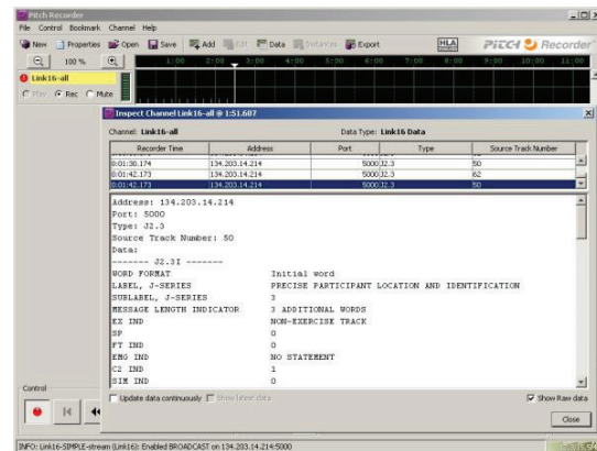
Figure 8: Screenshot of Pitch Recorder Link 16 recording.
