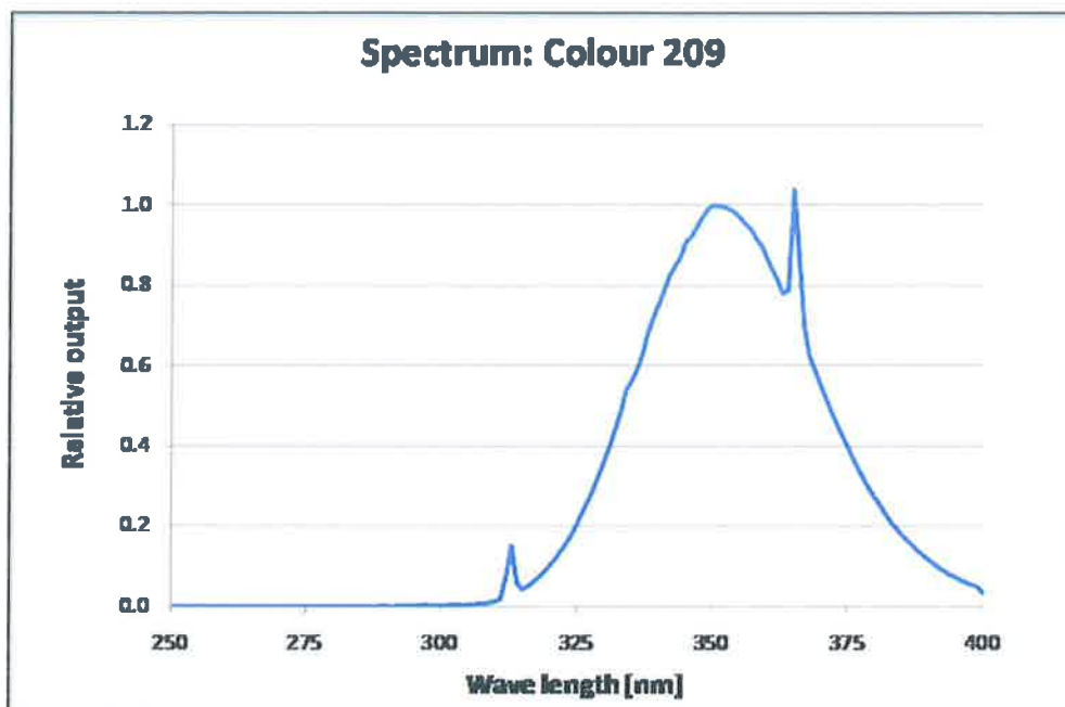
Figuur 41: Lichtspectrum Philips Cleo Compact 36W UV-A lampen [21]
