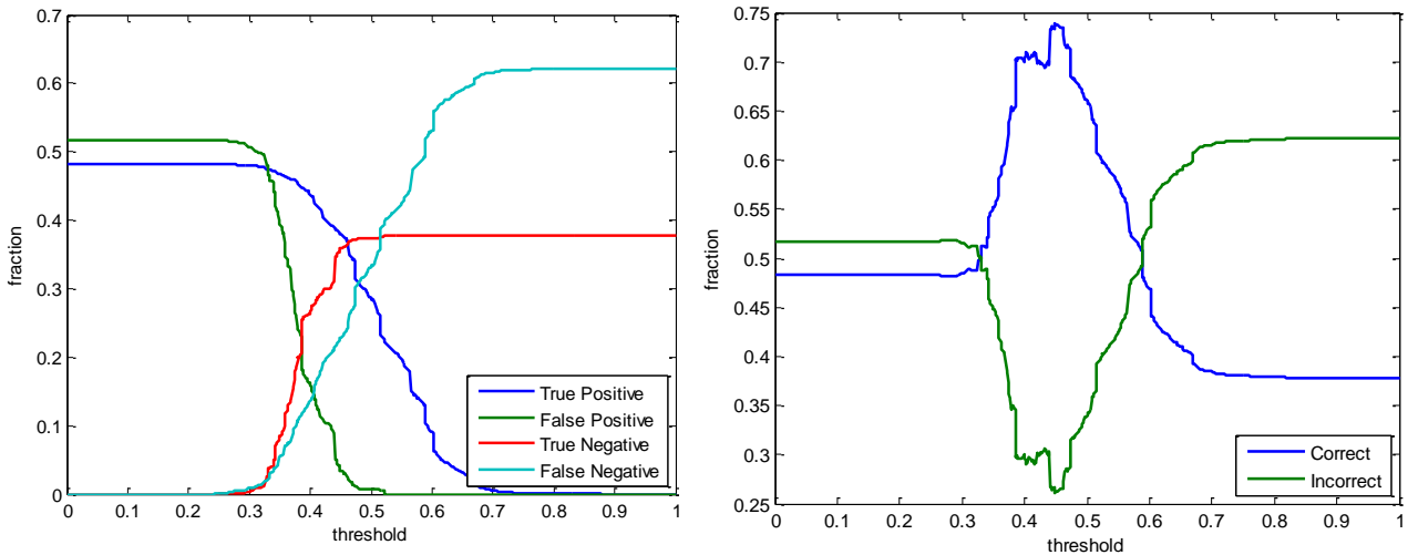
Figure 3: TP, FP, TN, FN, and the correct (TP+TN) and incorrect (FP+FN) for the alert system and different similarity thresholds.
