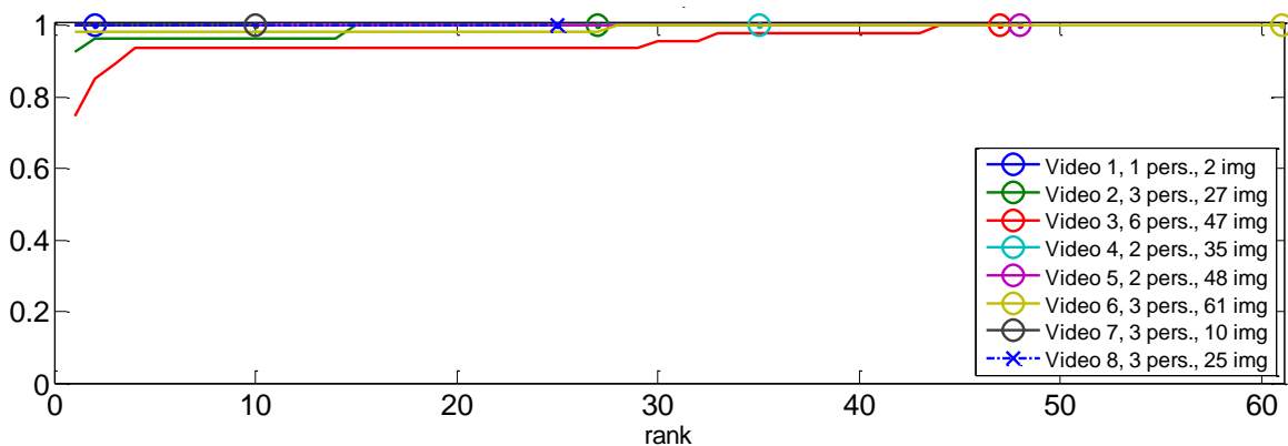
Figure 5: CMC curve of the best matches of the same person per video.
