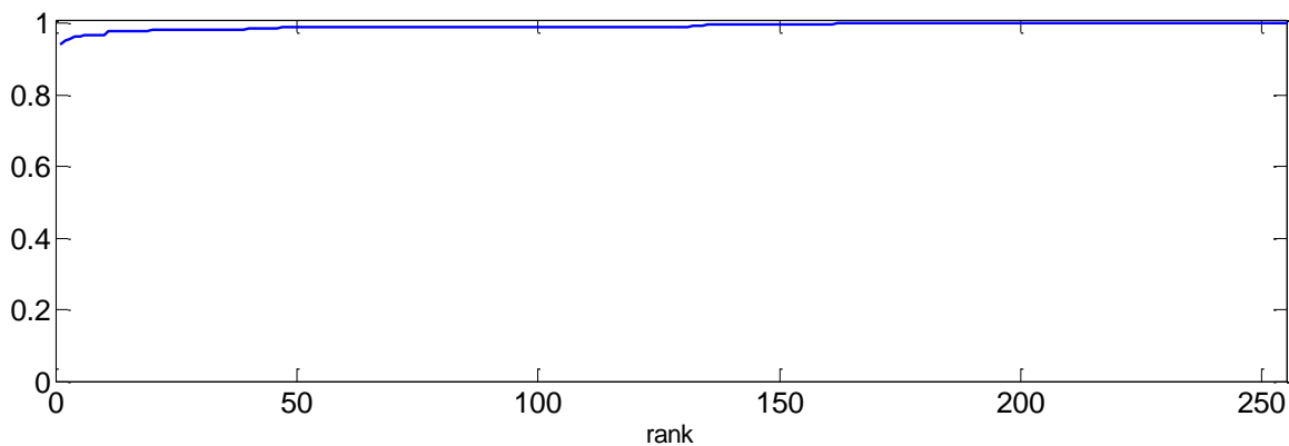
Figure 4: CMC curve of best matches over 23 persons and 255 tags in all videos.
