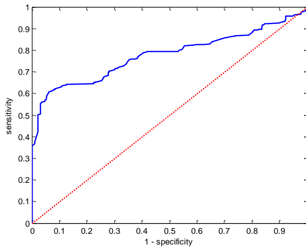
Figure 2: ROC curve of the alert system, which shows the sensitivity TP/(TP+FN) and specificity TN/(TN+FP) for various similarity threshold values.
