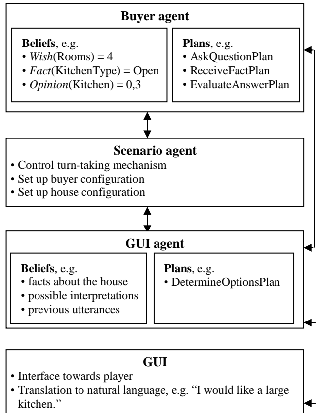
Figure 2. Agent architecture
