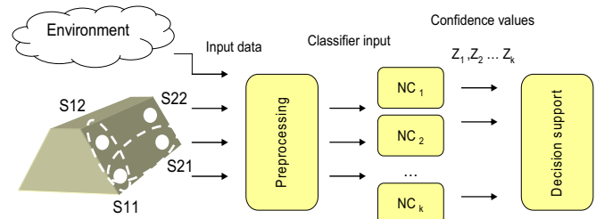
Fig. 2 Generic scheme of abnormality detection scheme
