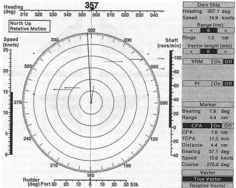
Figure 1. The ARPA navigation display. Collision avoidance information is presented on the right. Radar information is surrounded by vessel status information presented in scales. The position of the controlled vessel is the screen centre.
