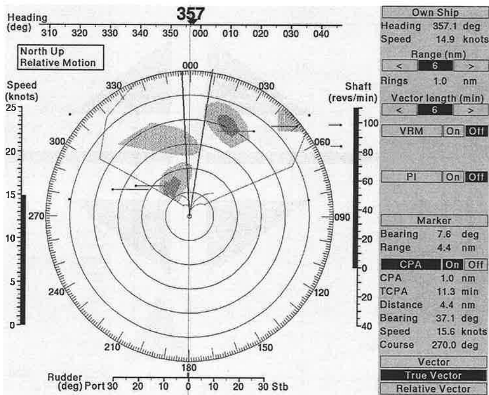
Figure 2. The ARPA/PCE/course navigation display. Baseline ARPA information is supplemented with PCE information: the vessel's heading line, the vessel's predicted track ahead (30 min prediction), the vessel's inherent manoeuvring area, and zones indicating areas with a passing distance to other traffic ships less than 1 nm. The dark zones represent areas with a passing distance less than 0.5 nm.
