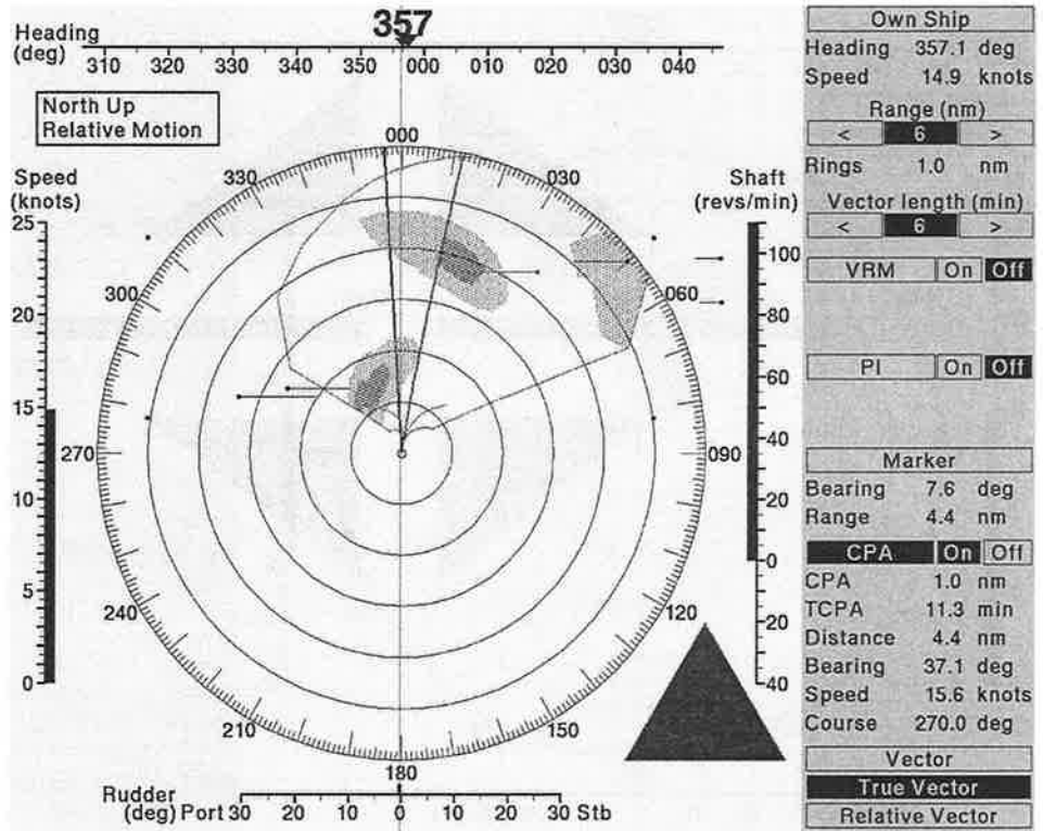
Figure 3. The ARPA/PCE/course/speed navigation display. The situation presented here represents a speed-trial with Shaft 80 revs/min. A triangle appears on the screen as a reminder that the speed-trial function is active.
